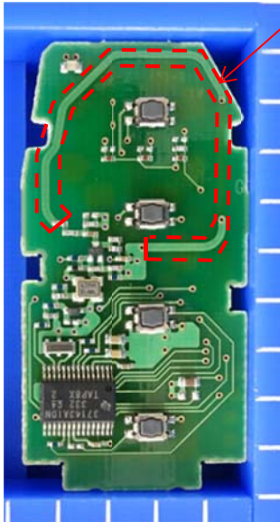
4-Button type
