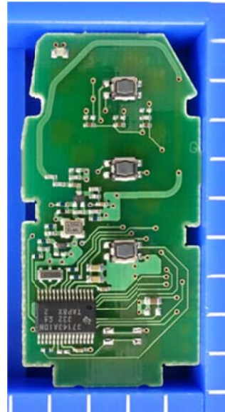
3-Button type
