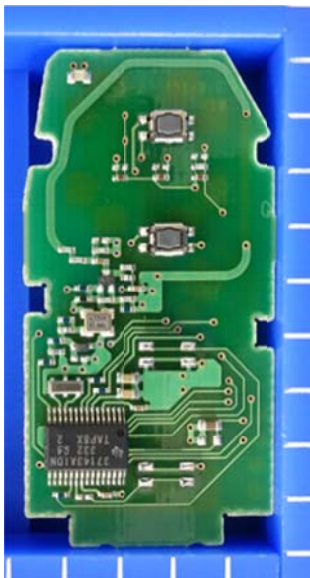
2-Button type
