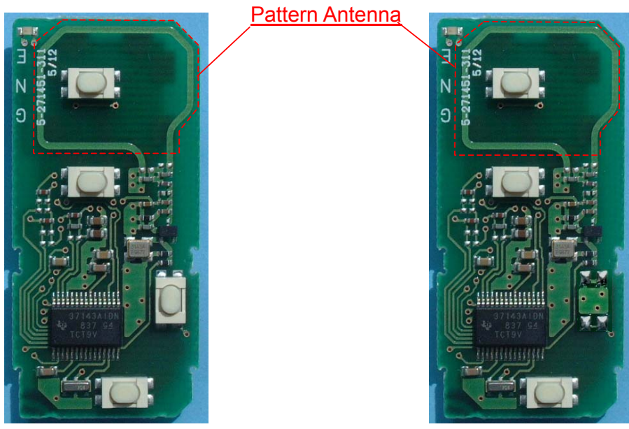
4 switches type
