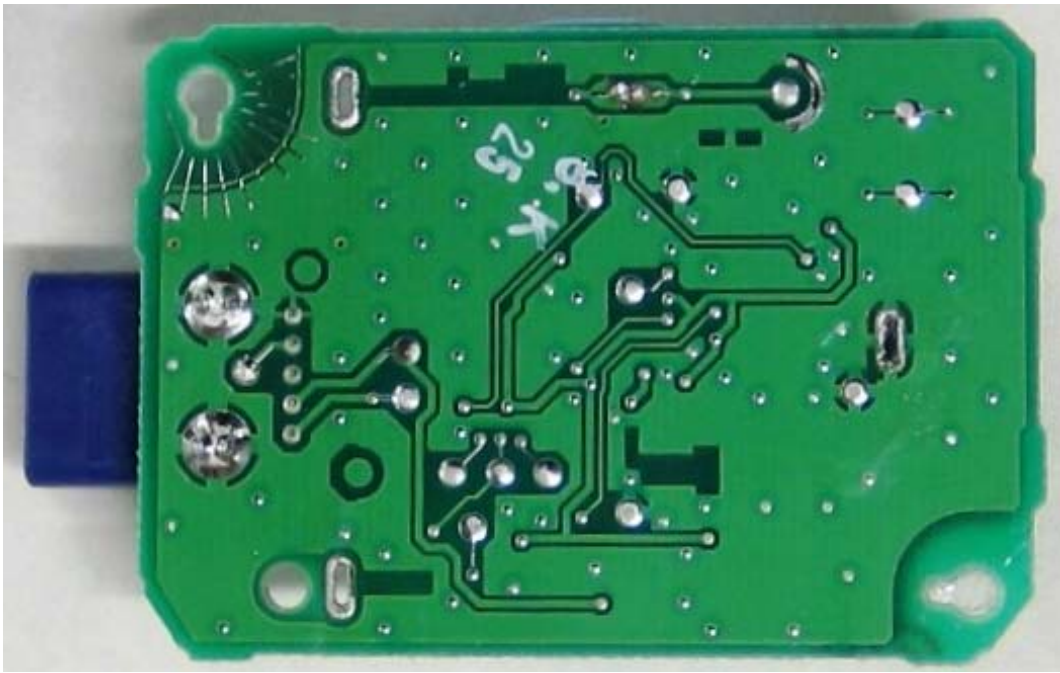
Solder Side
