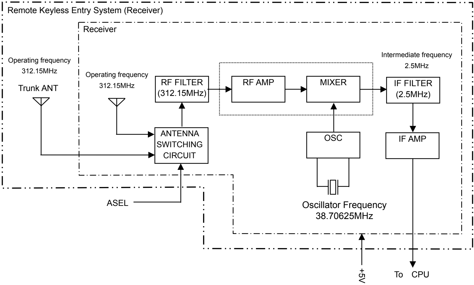
Fig. Block diagram of Remote Keyless Entry System
