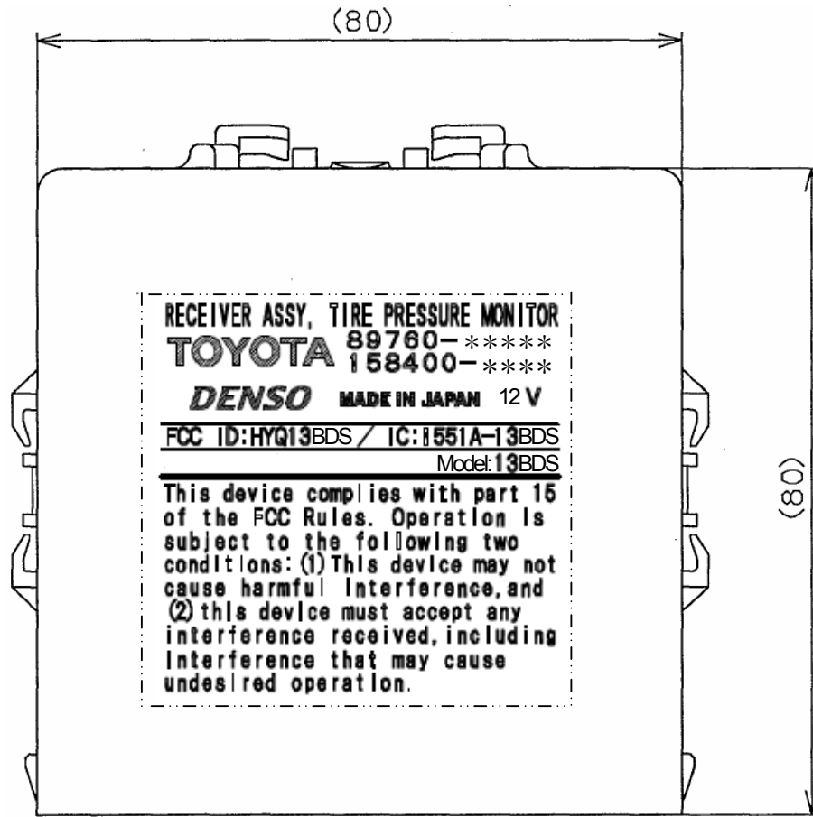
Fig. Marking location and layout of Receiver
