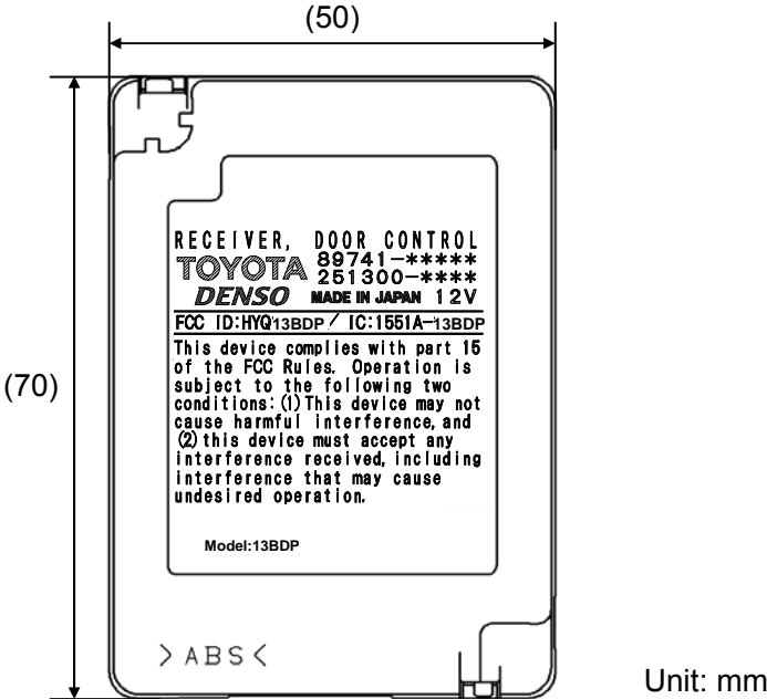
Fig. Marking location and layout of Receiver
