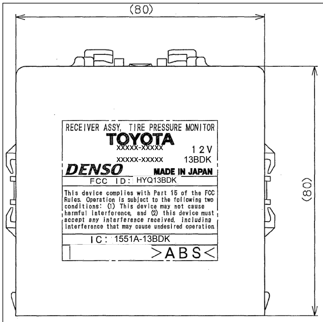
Fig. Marking location and layout of Receiver
