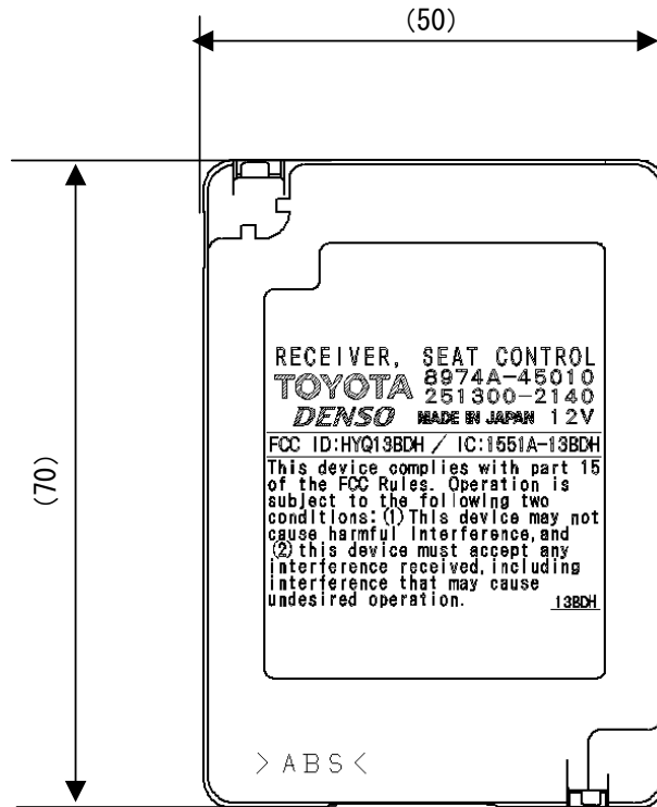
Fig. Marking location and layout of Receiver
