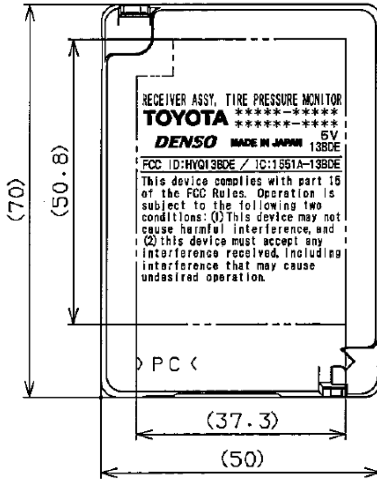
Fig8.1. Marking location and layout of receiver
