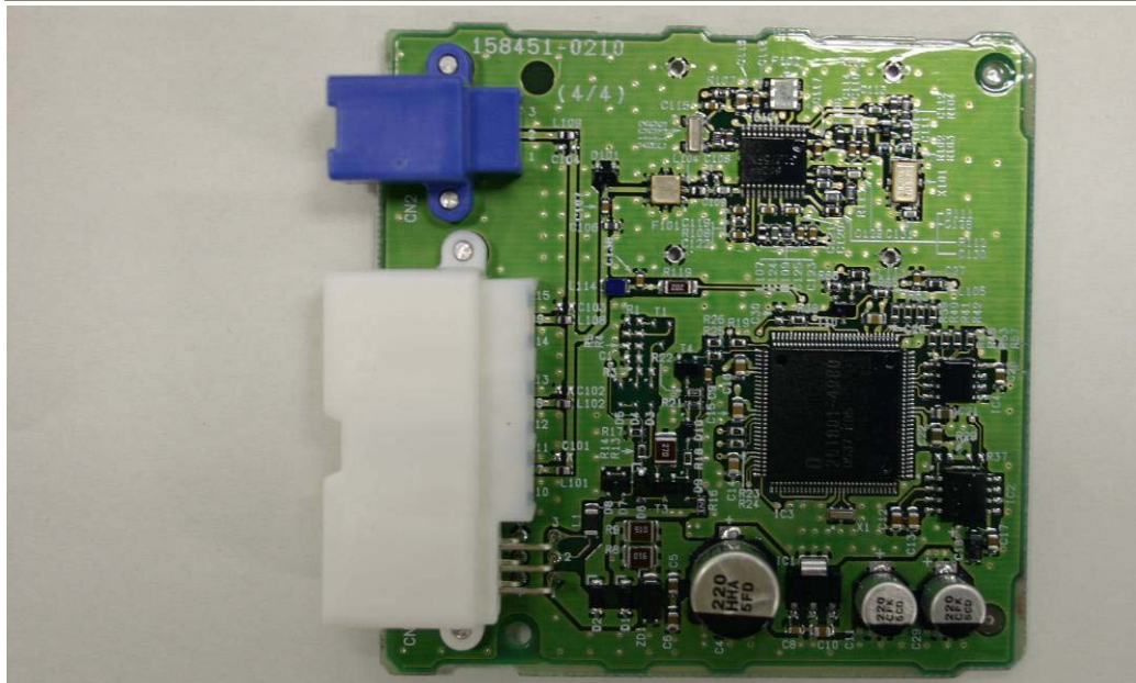
Component Side
