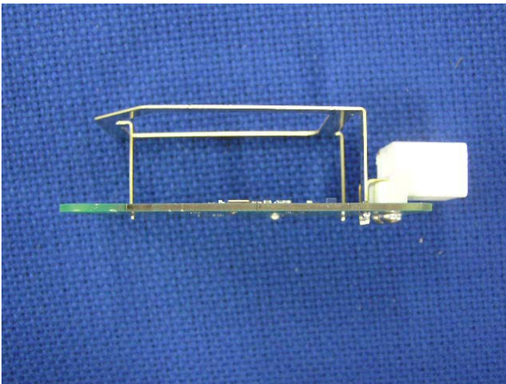
Inside side without shield
