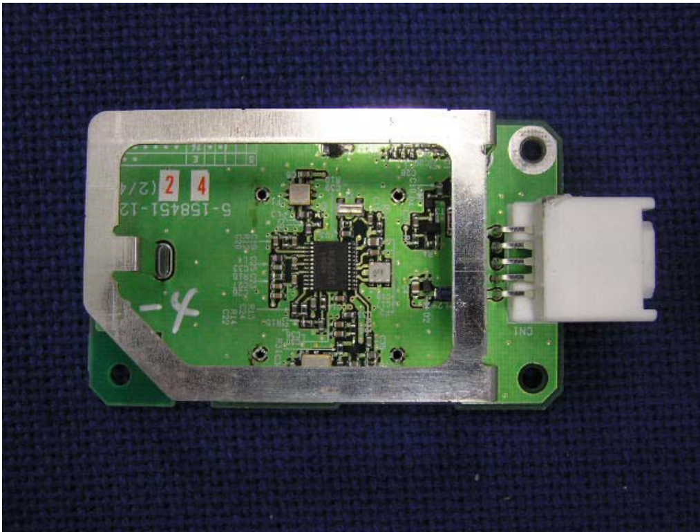
Comp side without shield
