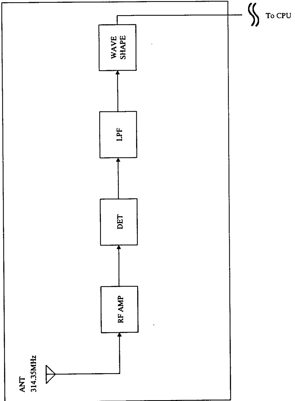
Fig. Block diagram of receiver
