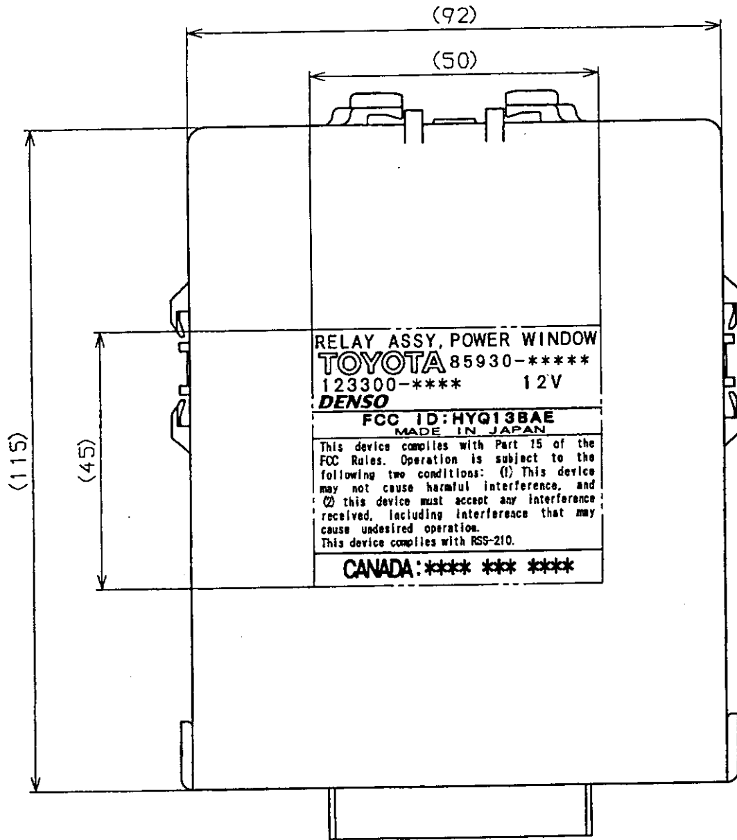
Fig.5 Marking layout for receiver
