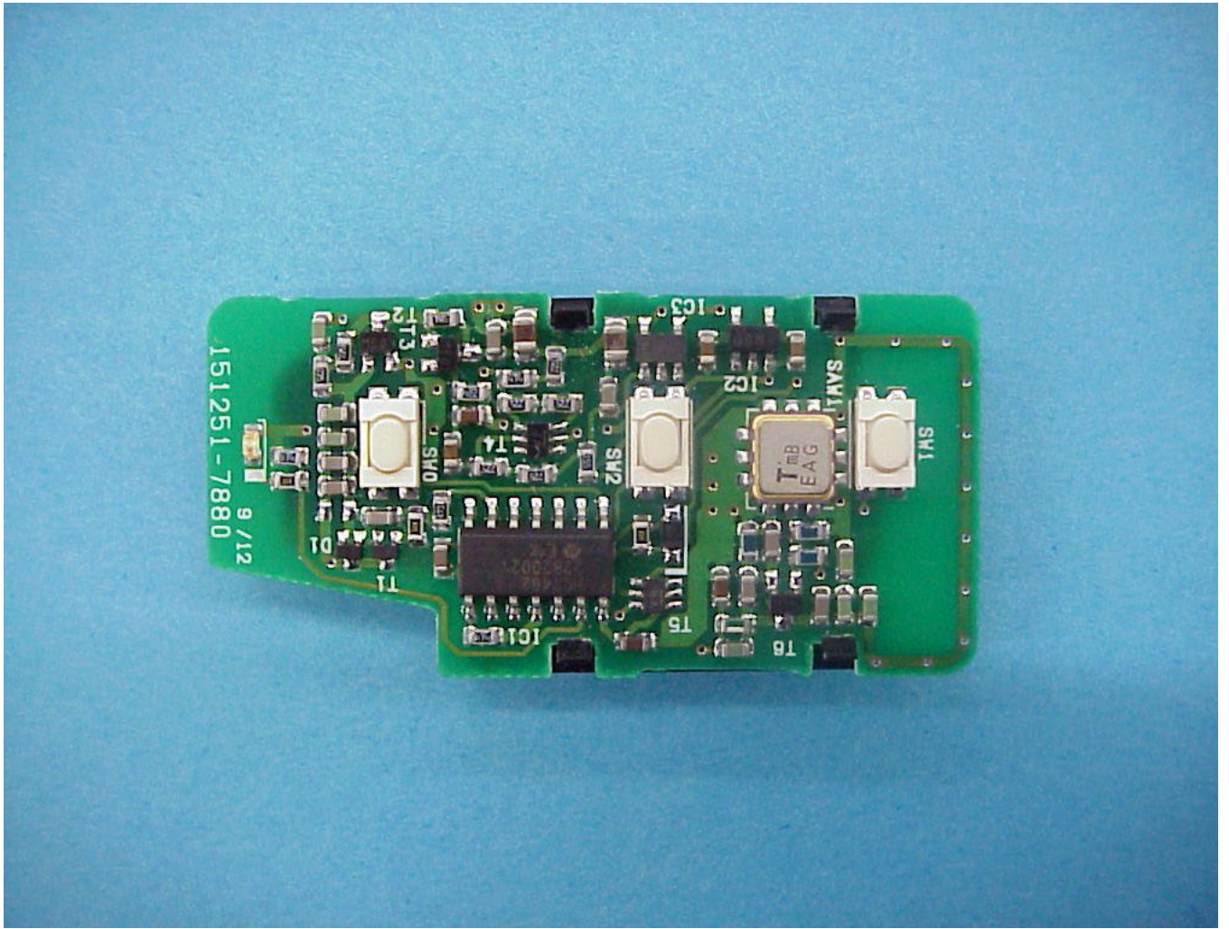
Top of PCB – silver parts are not removable - component side with view of TX
