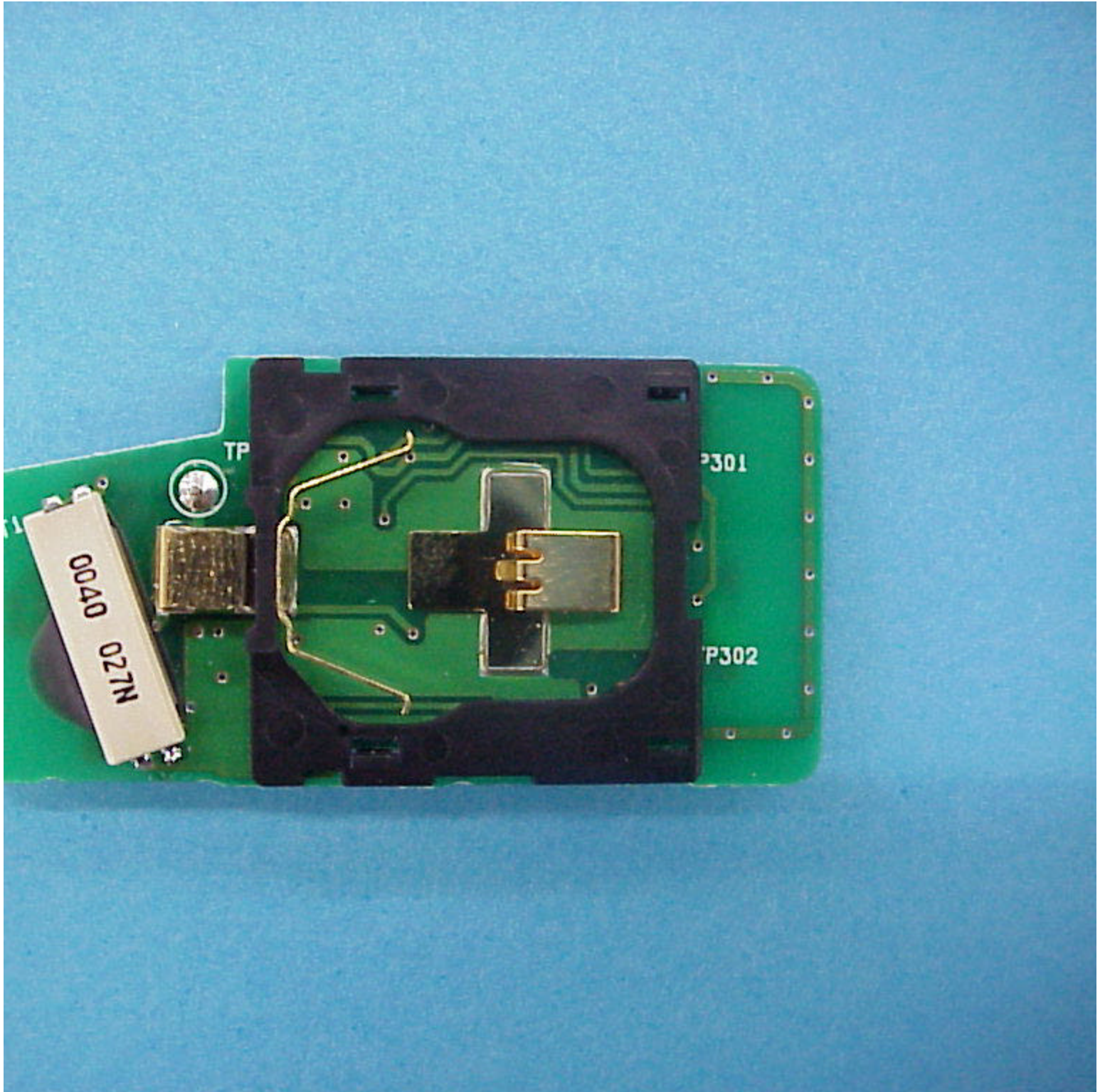
PCB solder side without battery view of tx
