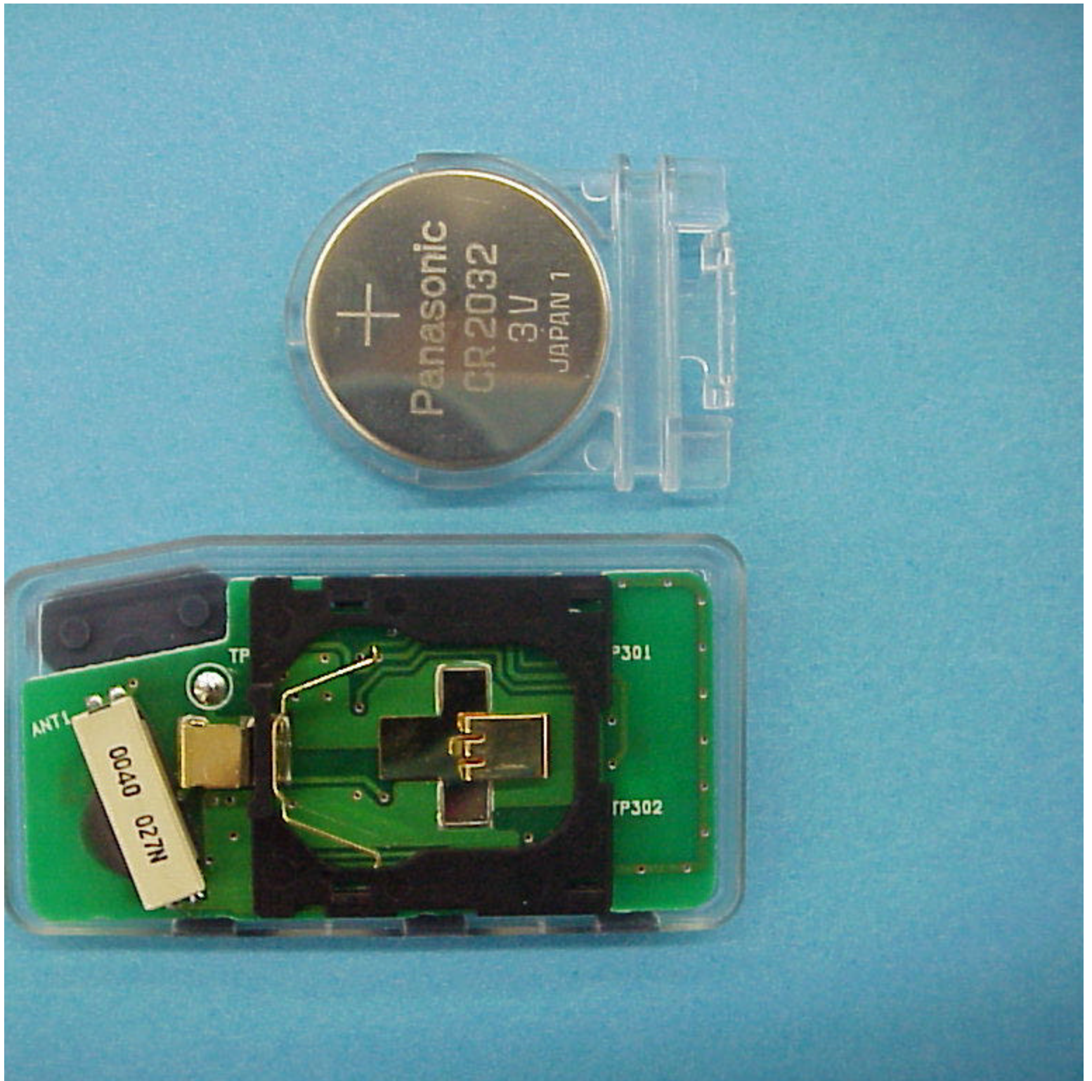
PCB solder side with battery view of tx
