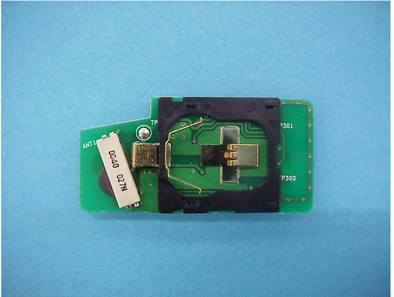
PCB solder side without battery
