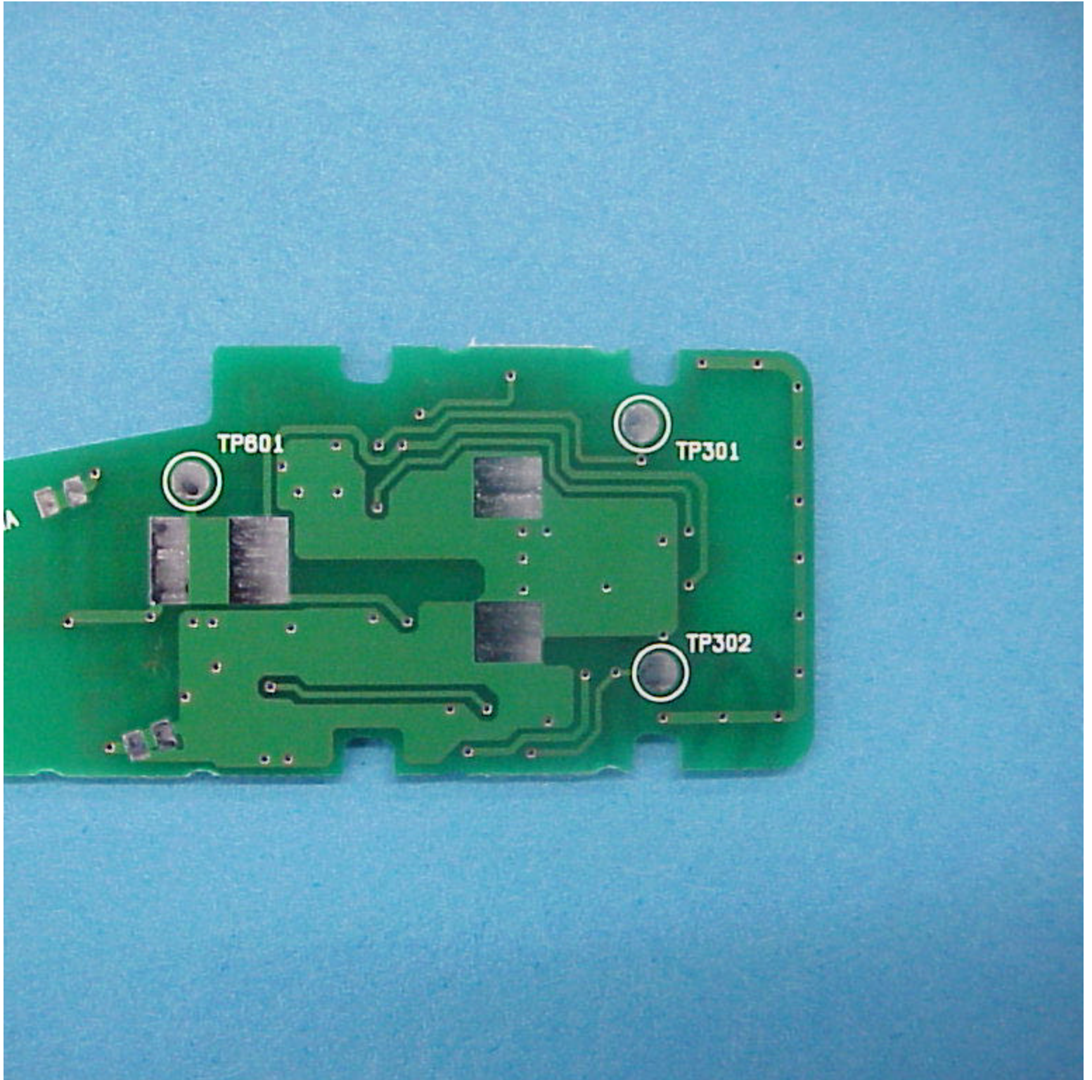
PCB solder side without battery and terminal view of tx
