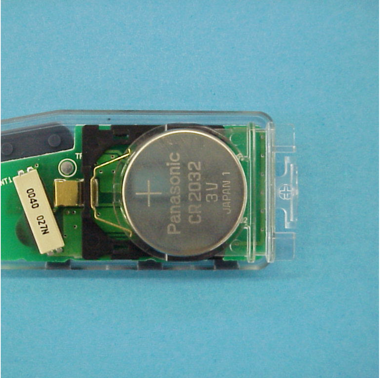
PCB with battery
