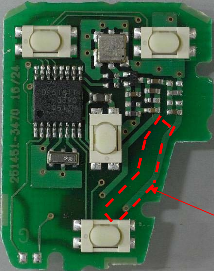
Comp. Side (4-button)
