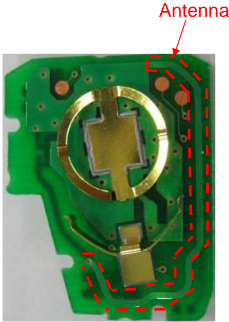
Sold. Side (Plated with gold)
