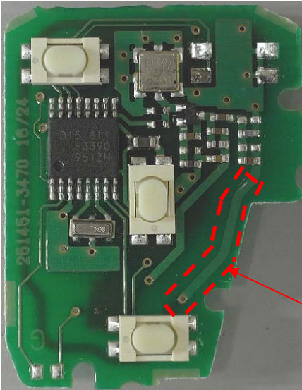
Comp. Side (3-button)
