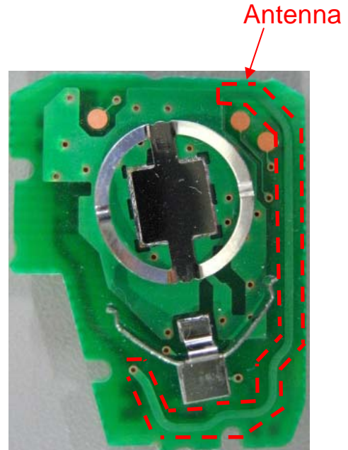
Sold. Side (Plated with nickel)
