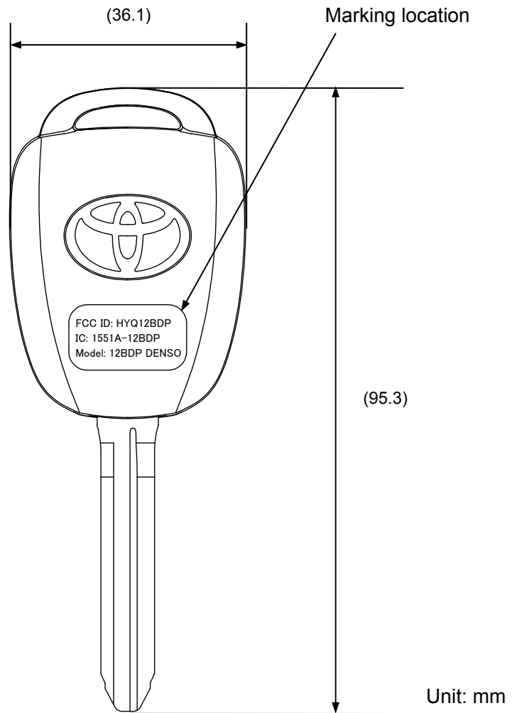
Fig. Marking location and layout of Transmitter
