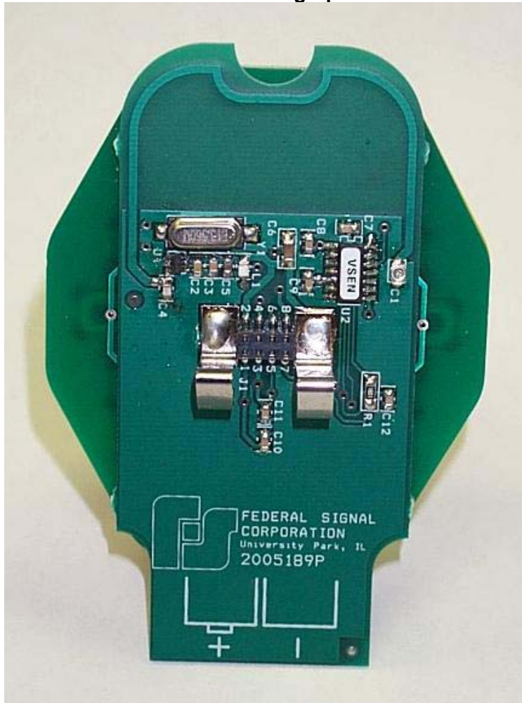
Photograph of RF Board – Component & Foil Side
