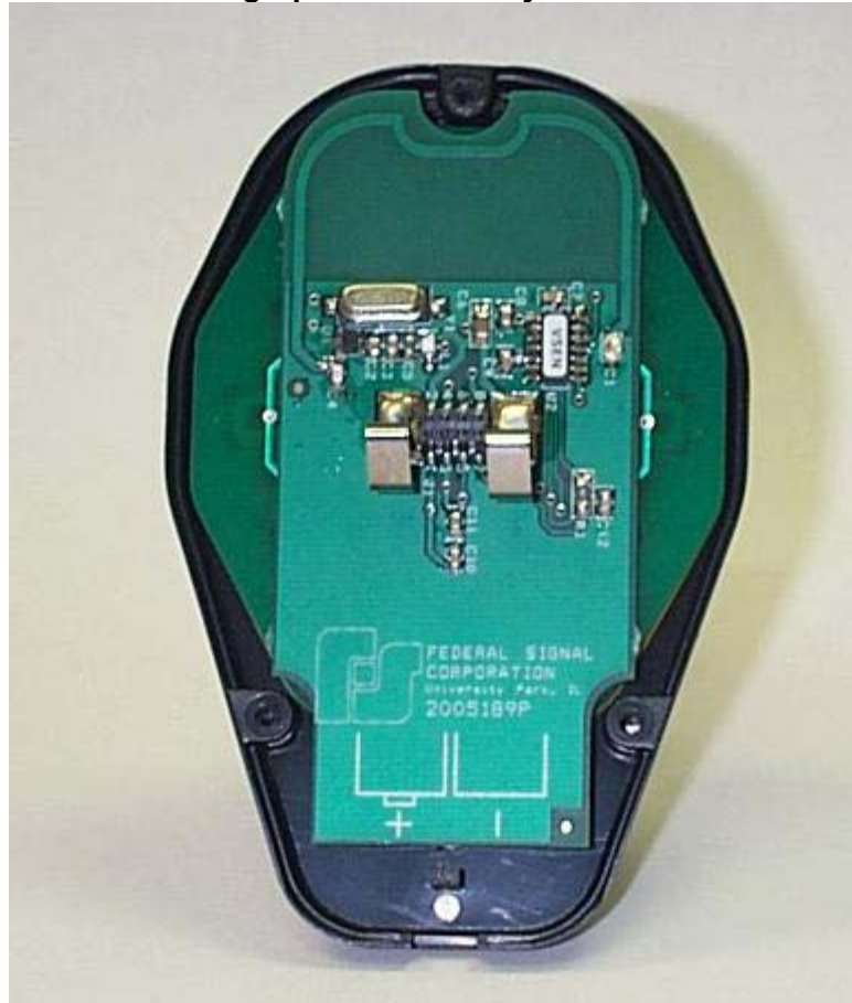
Photograph EUT Partially Assembled
