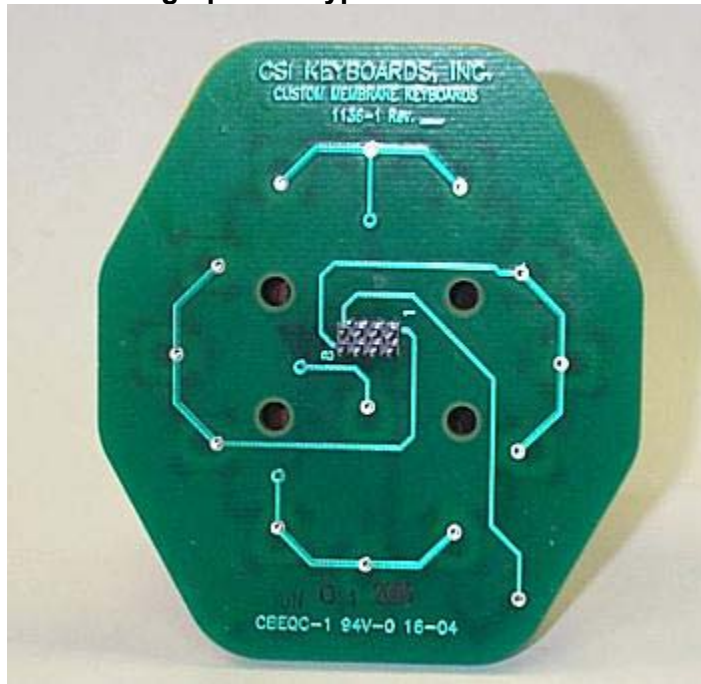
Photograph of Keypad Board – Foil Side
