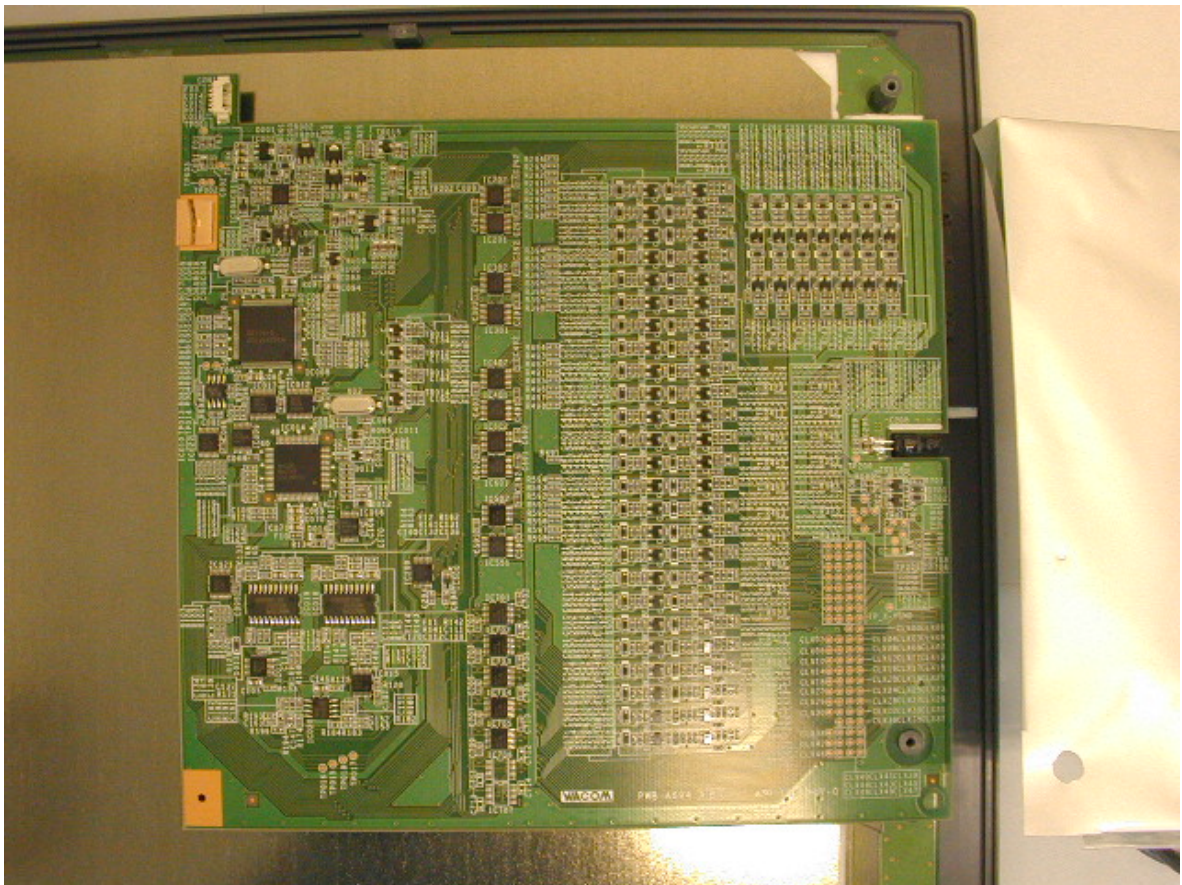
Photo-4 Surface of Control board (PTZ-1230)
