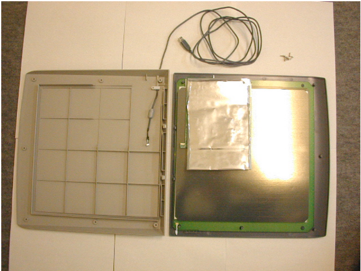
Photo-3 Bottom cover removed (PTZ-1230)
