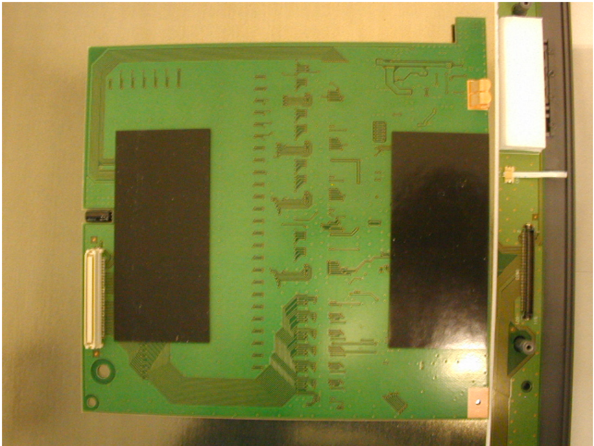
Photo-5 Reverse of Control board (PTZ-1230)
