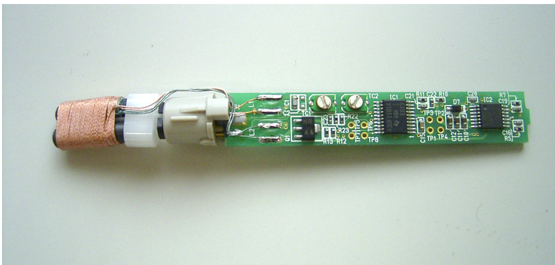
Photo A-14 Internal view _ Maker Pen (model: ZP-600)
