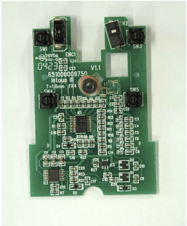
Photo A-18 Surface of internal board _ 2D Mouse (model: ZC-100)
