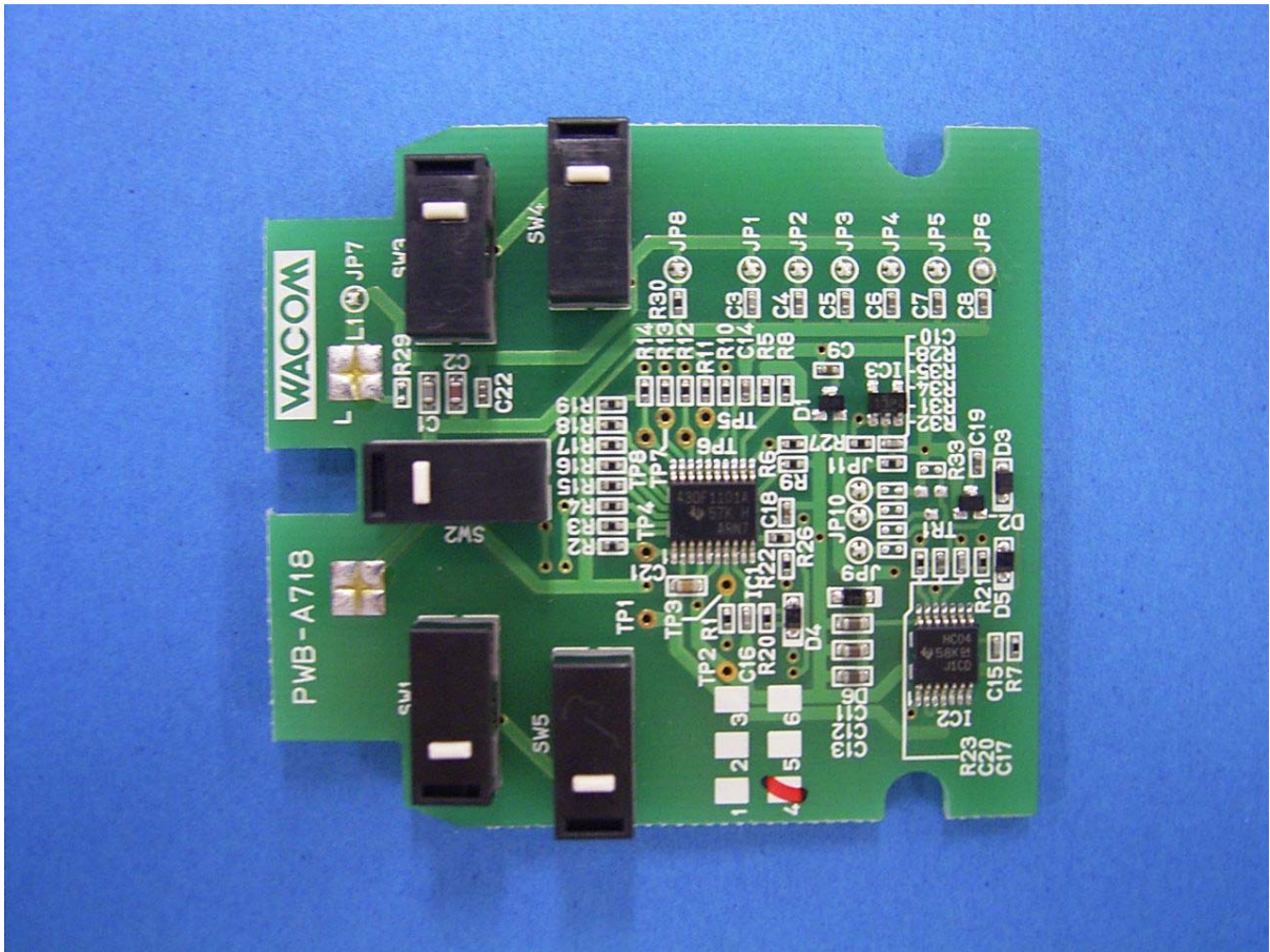
Photo A-22 Surface of internal board _ Lens Cursor (model: ZC-210)
