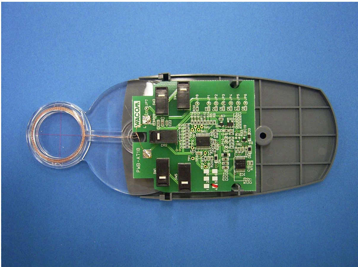
Photo A-21 Internal view _ Lens Cursor (model: ZC-210)
