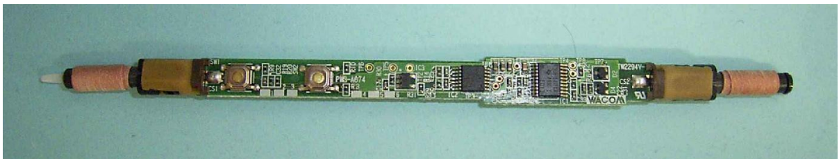
Photo A-5 Internal view _ Classic Pen (model: ZP-300E)
