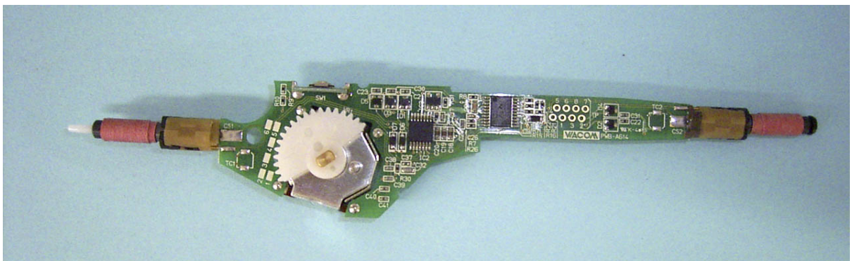
Photo A-8 Internal view _ Airbrush (model:ZP-400E)
