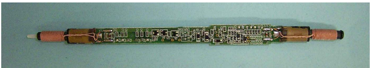
Photo A-6 Internal view _ Classic Pen (model: ZP-300E)
