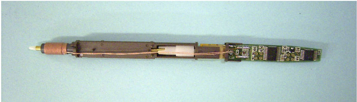
Photo A-2 Internal view _ Ink Pen (model: ZP-130)
