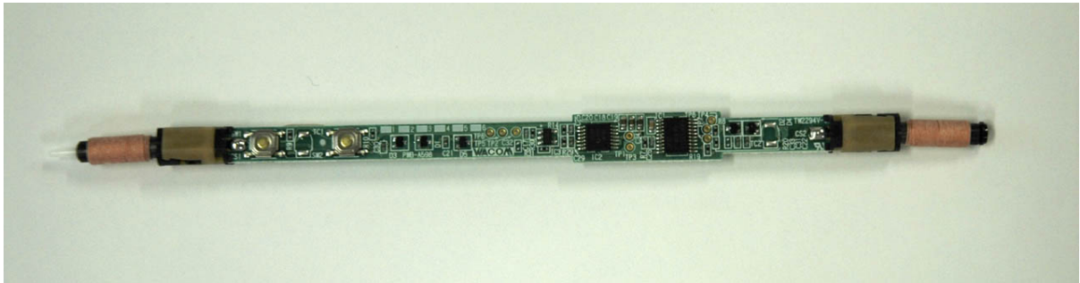
Photo A-11 Internal view _ Grip Pen (model: ZP-501E)
