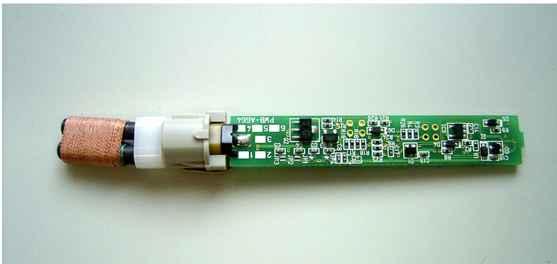
Photo A-15 Internal view _ Maker Pen (model: ZP-600)
