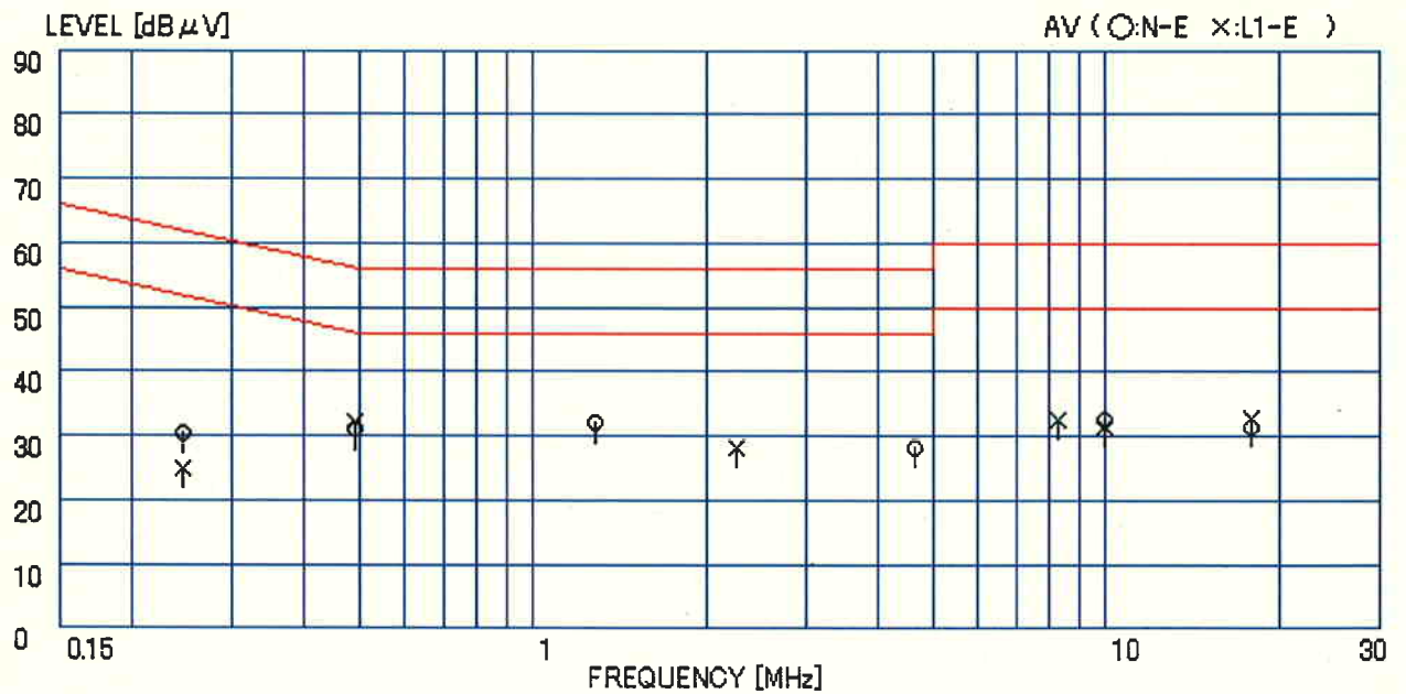
<Average Measurement>
