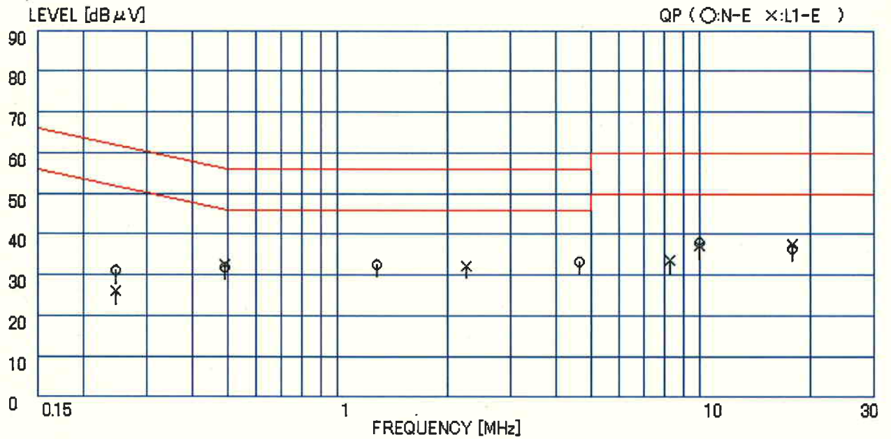
<Q-Peak Measurement>
