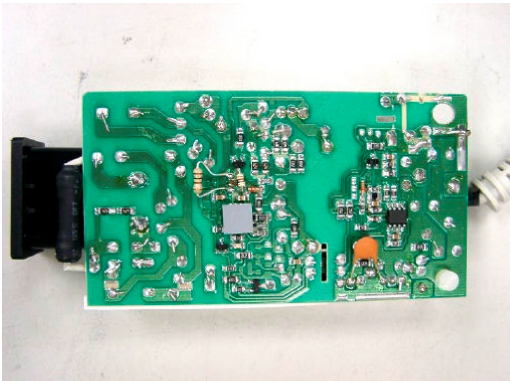
30. Rear view of PCB 8 (Adaptor)
