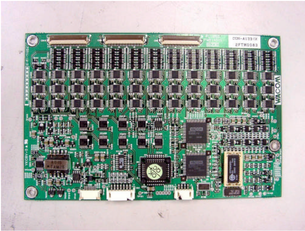
15. Front view of PCB 2 (Monitor)
