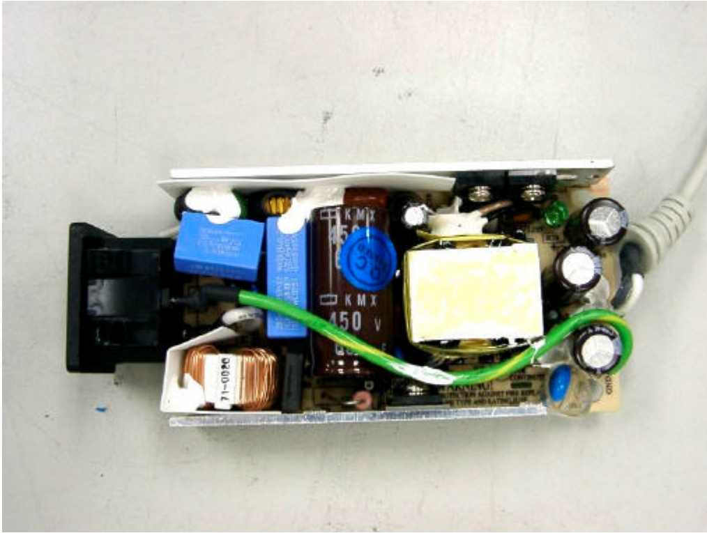
29. Front view of PCB 8 (Adaptor)
