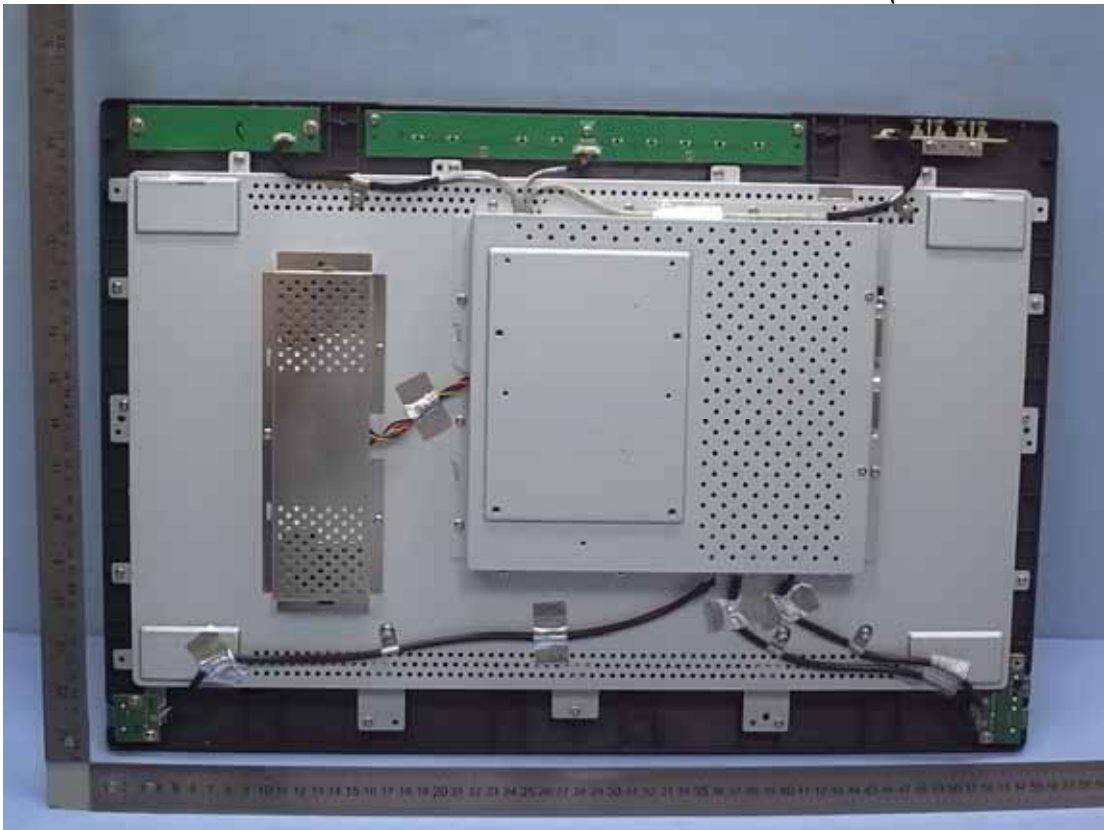
Figure 13 Internal View (Back Cover Removed)
