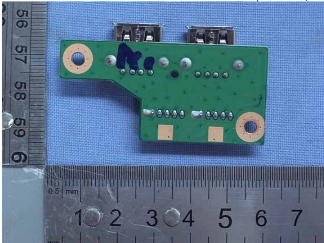
Figure 17 Internal View (USB Board, Back View)
