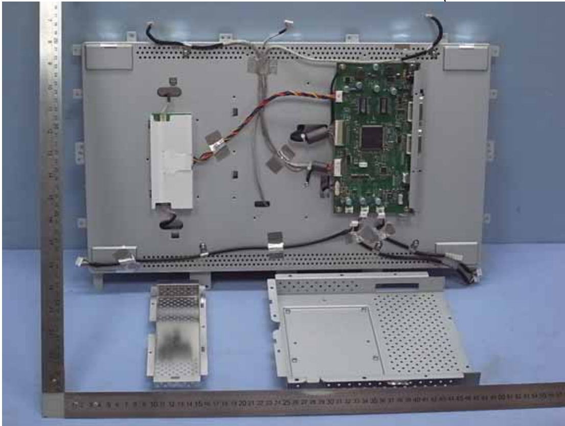
Figure 25 Internal View (Removed Main Board & Inverter Board)
