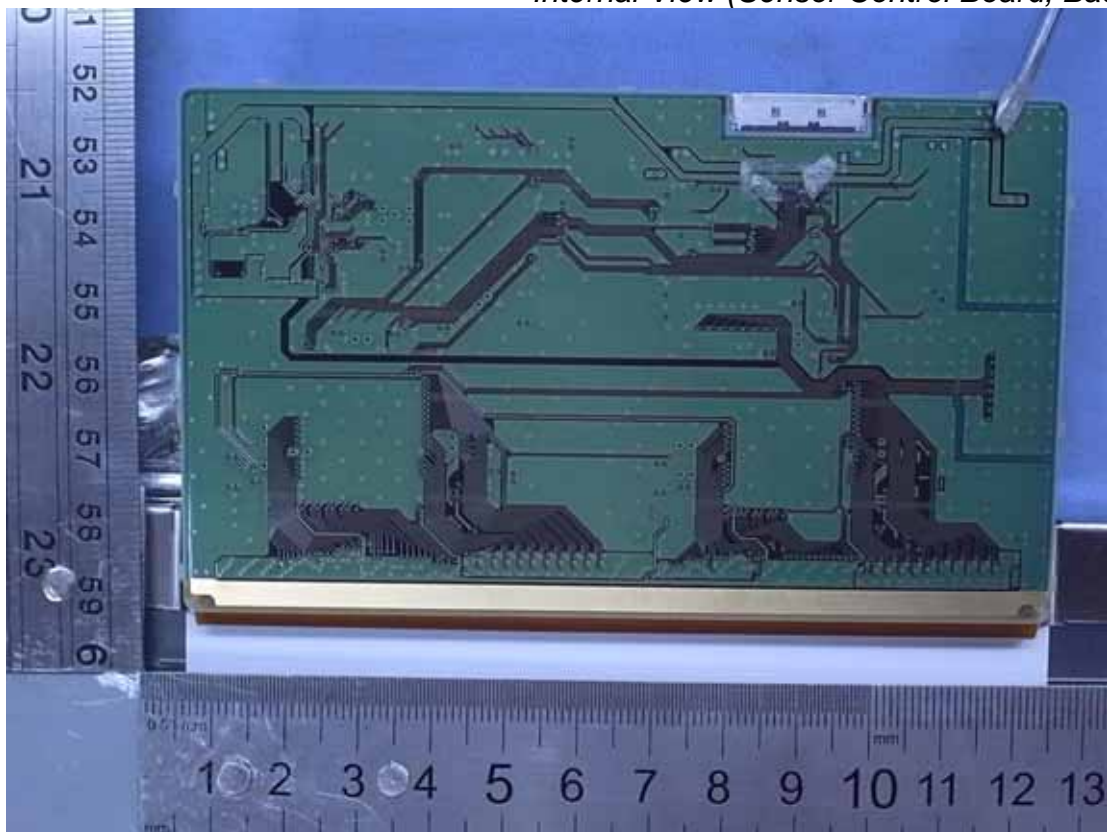
Figure 35 Internal View (Sensor Control Board, Back View)
