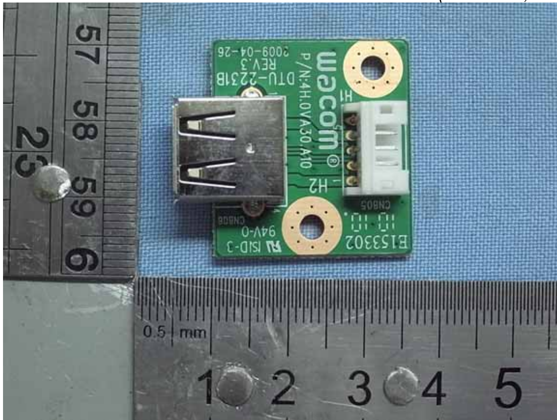
Figure 15 Internal View (USB Board, Back View)
