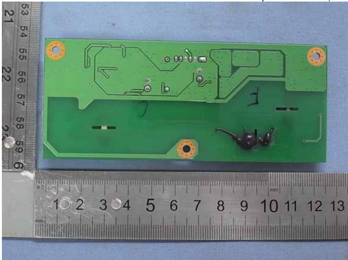
Figure 29 Internal View (Inverter Board, Back View)
