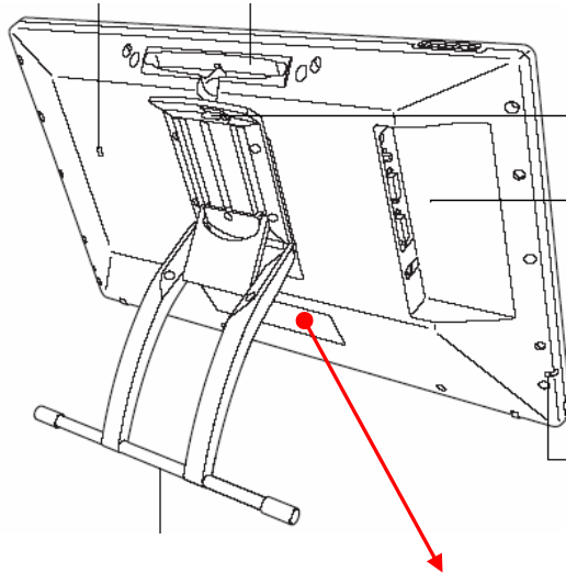
FCC Label Placement Location
