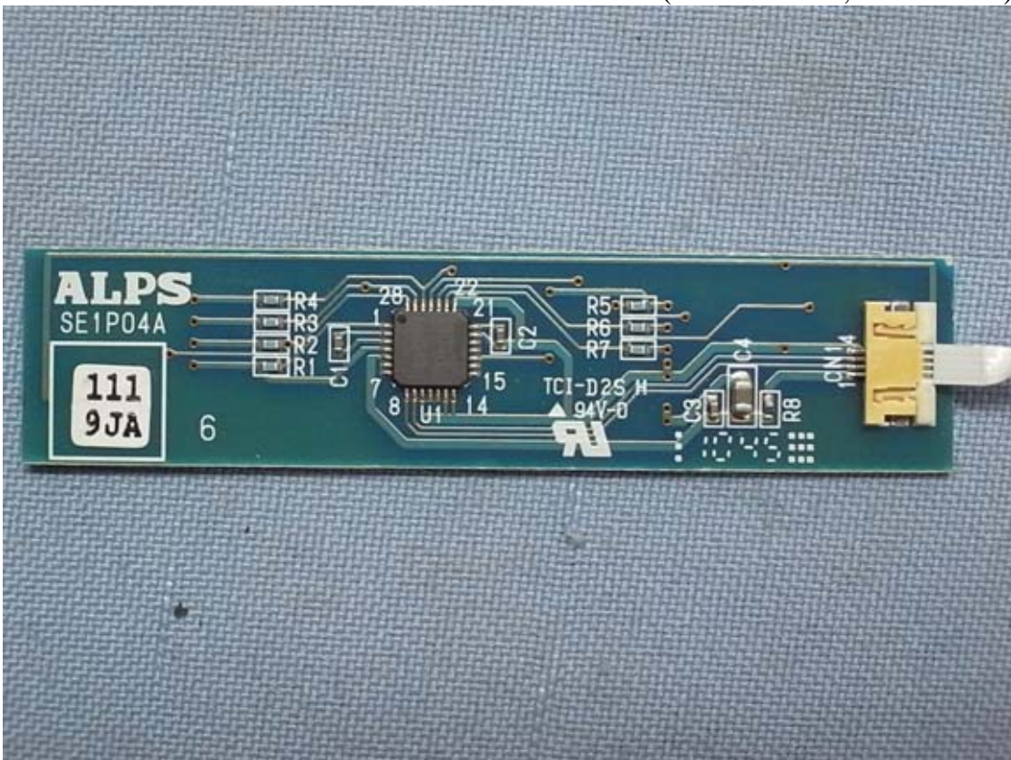
Figure 48 Internal View (Sensor Board, Front View)
