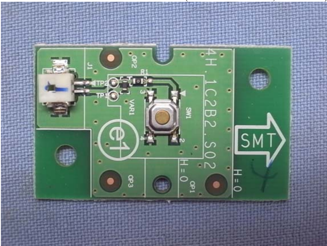
Figure 42 Internal View (Power Switch Board, Front View)
