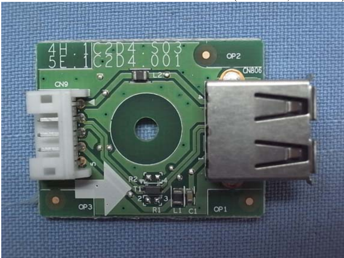
Figure 44 Internal View (USB Board, Front View)
