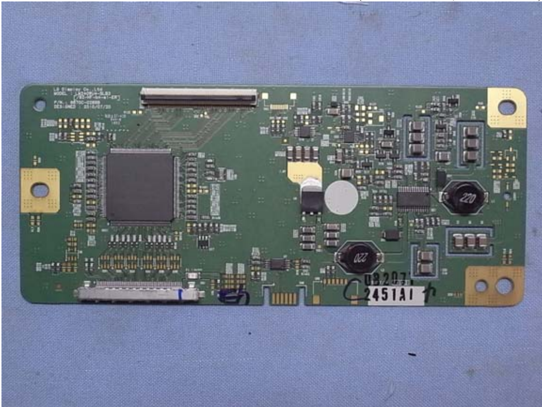
Figure 35 Internal View (LVDS Board, Front View)
