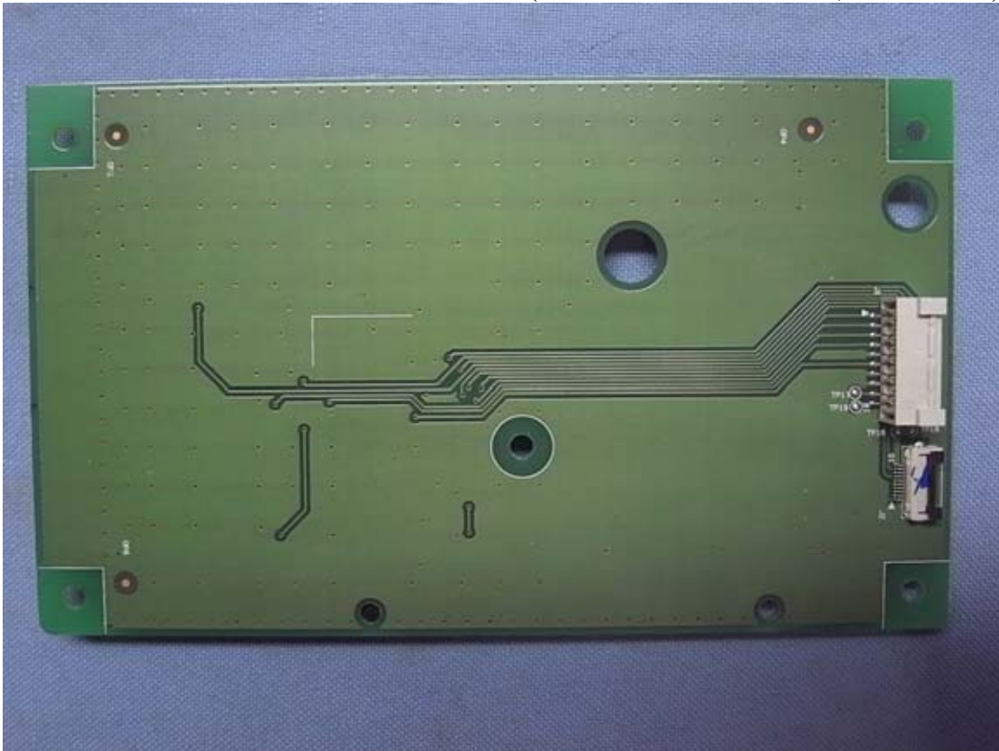
Figure 41 Internal View (Function Control Board, Back View)
