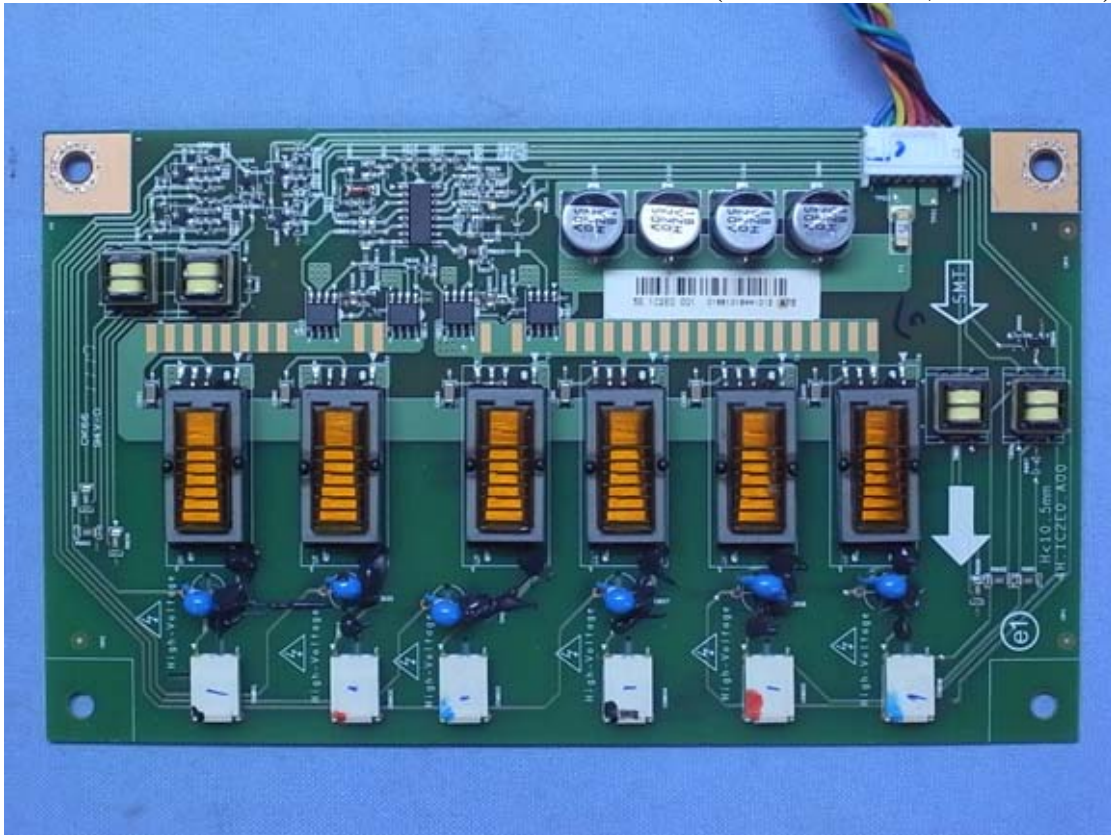
Figure 33 Internal View (Inverter Board, Front View)
