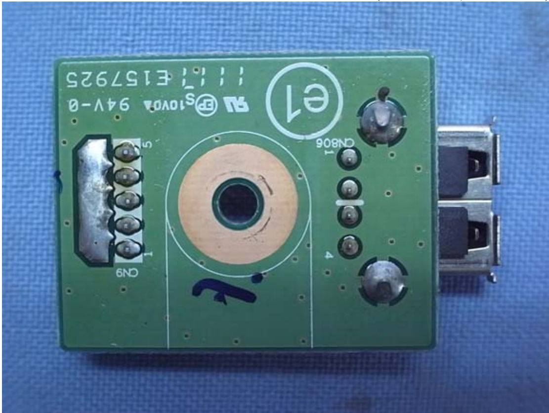
Figure 45 Internal View (USB Board, Back View)
