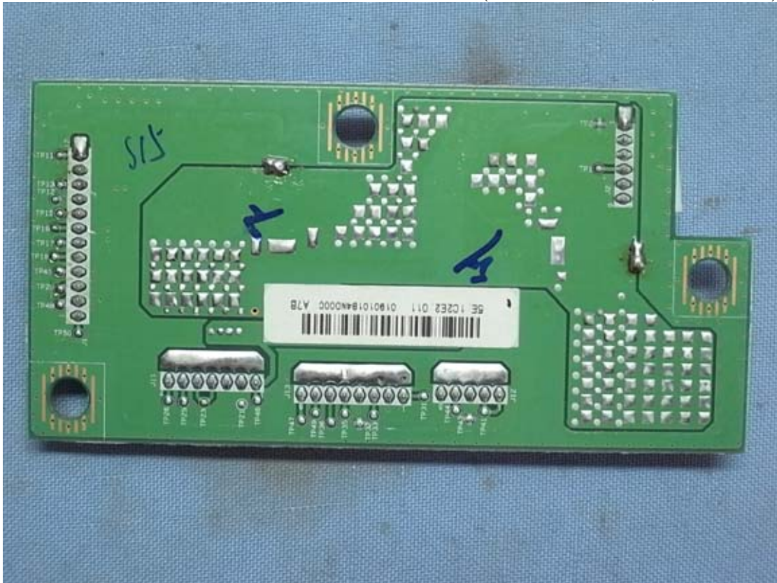
Figure 27 Internal View (Converter Board, Back View)
