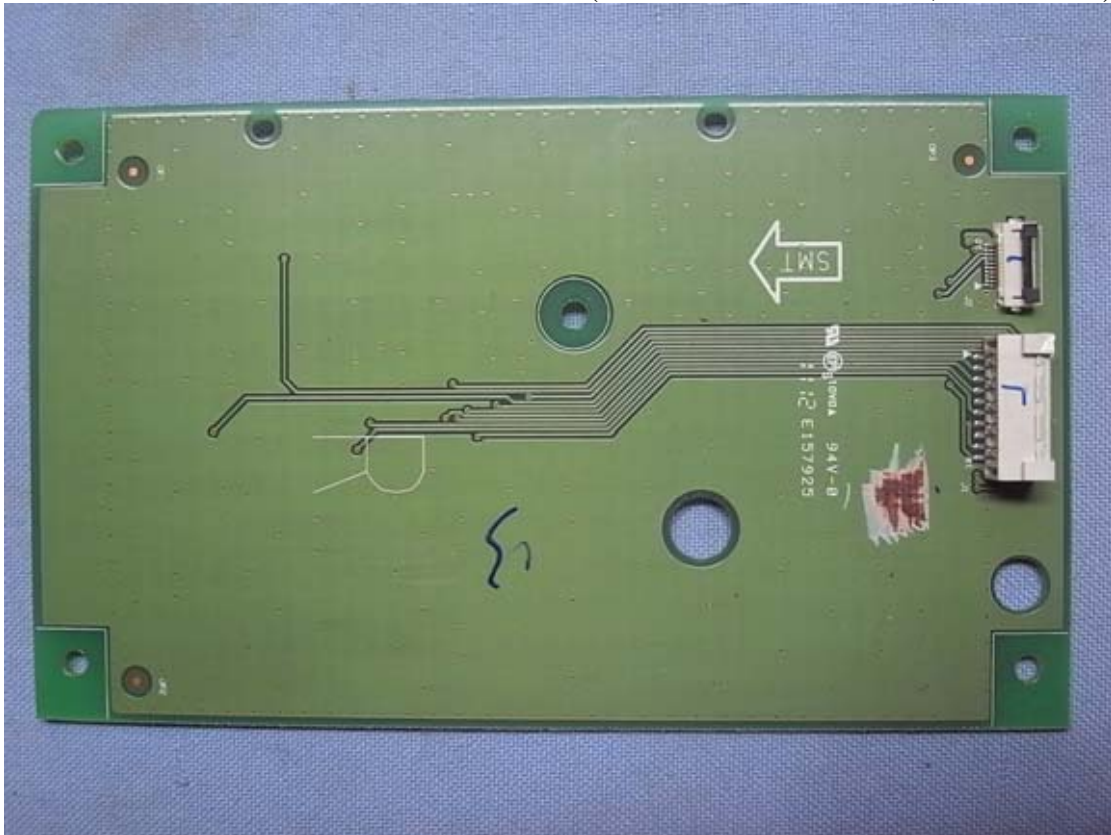
Figure 39 Internal View (Function Control Board, Back View)
