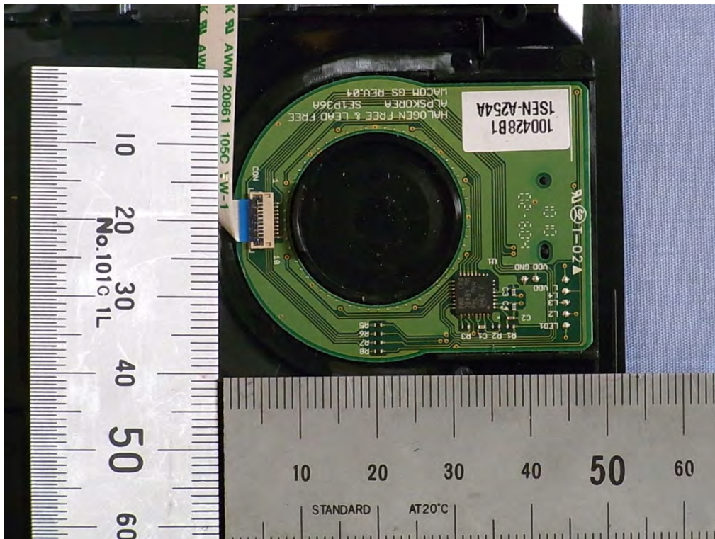
[TOUCH RING PWB (R)]
