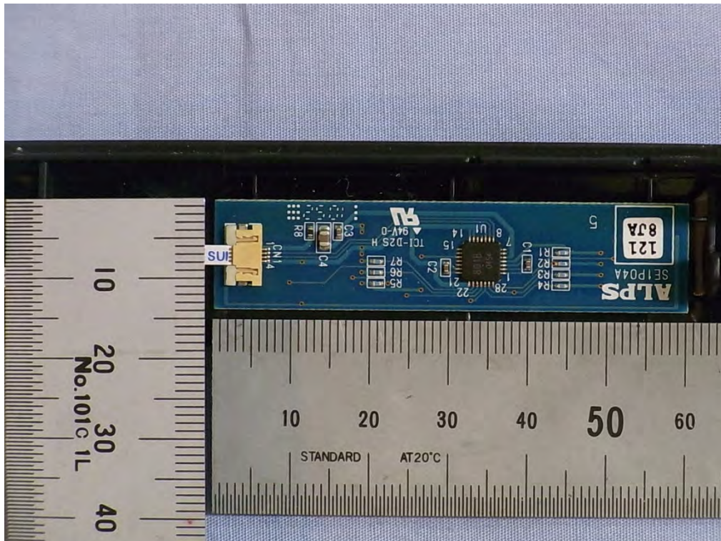
[TOUCH STRIP PWB]
