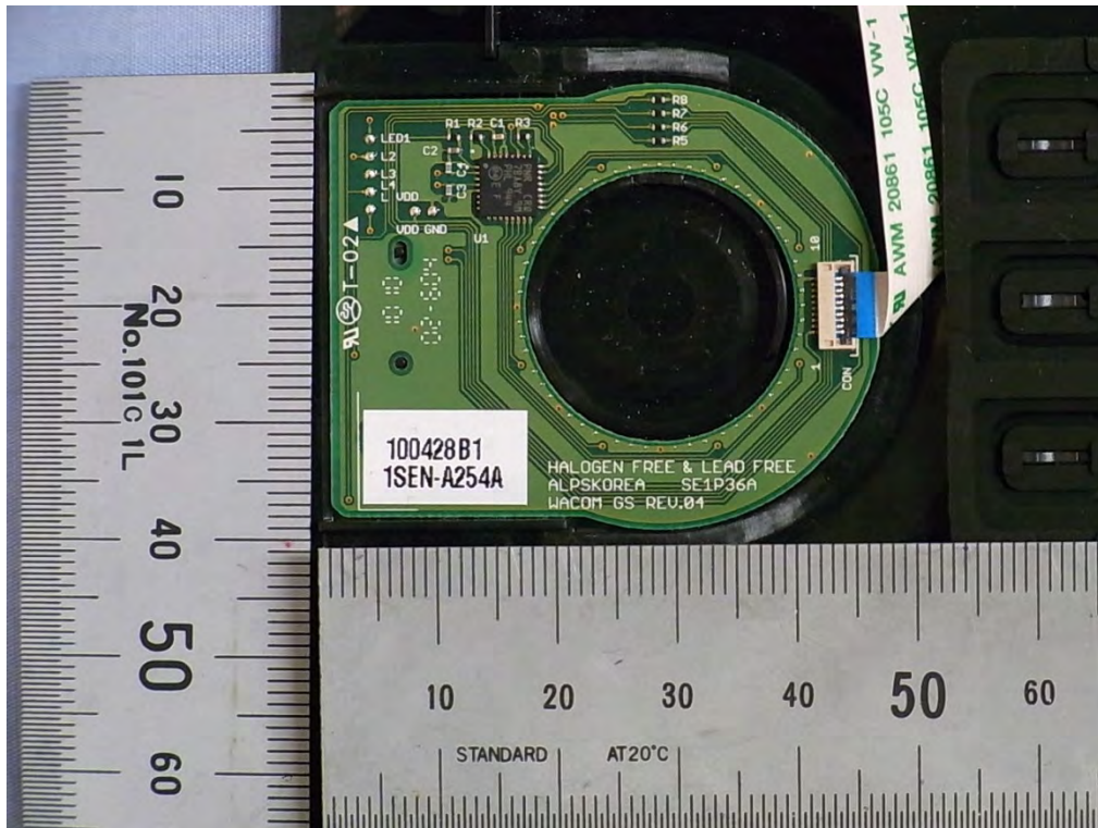
[TOUCH RING PWB (L)]
