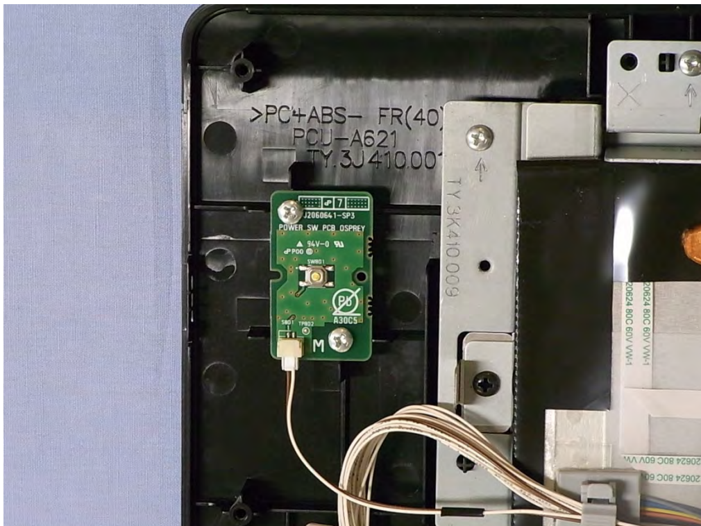
[Power SW PWB]
