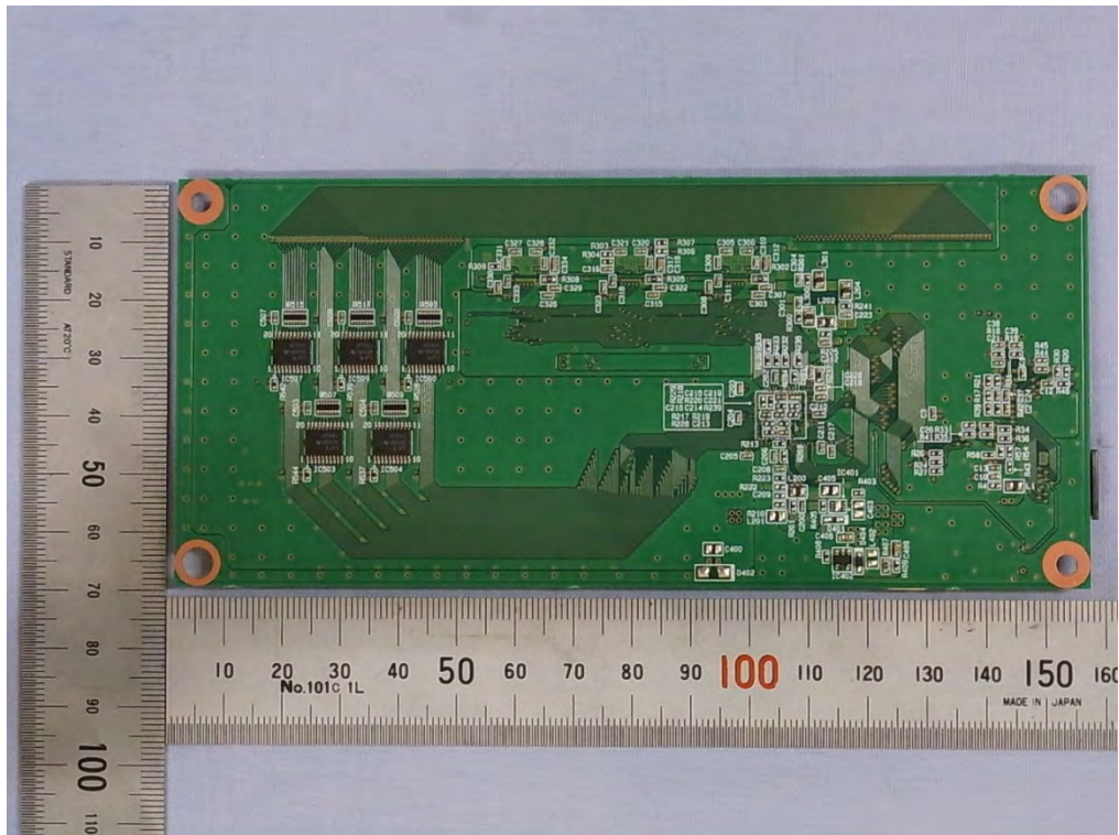
[TOUCH CONTROL PWB]
