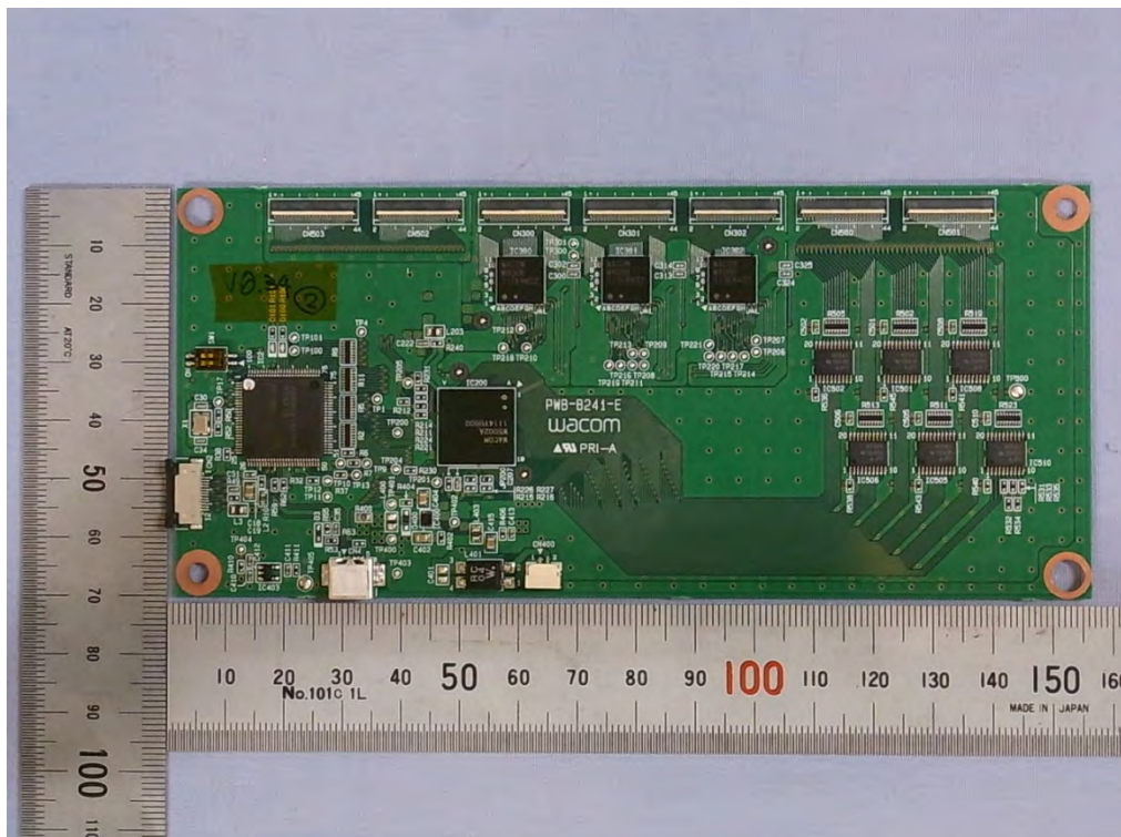
[TOUCH CONTROL PWB]
