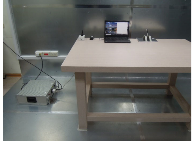
FCC_EMR_Conduction_Setup
