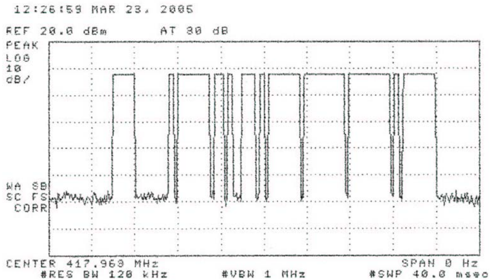
Figure 6.1. Transmissions modulation characteristics: (top) complete transmission, (bottom) expanded word (2.0 ms pulse followed by 26.0 ms of code).
