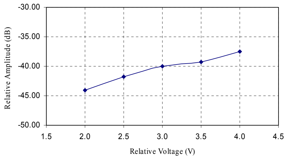
Figure 6.5. Relative emission at 418.0 MHz vs. supply voltage (pulsed emission).
