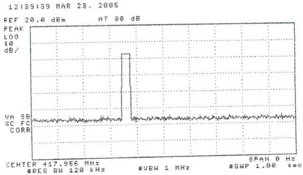
Figure 6.4. Transmitter 5 sec. transmission limit verification
