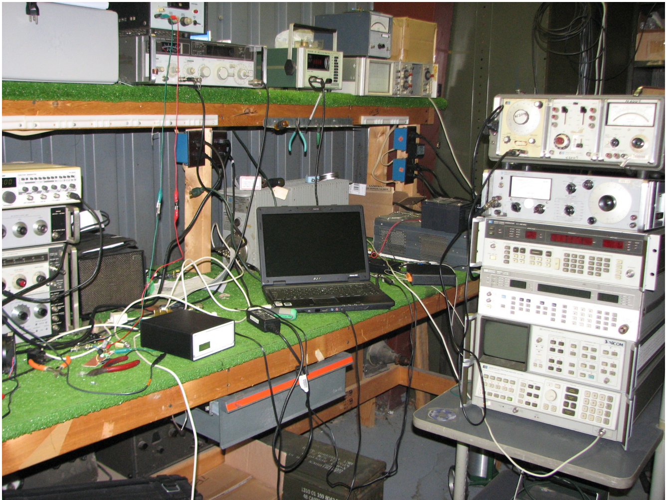
Engineering Laboratory, Test Setup for MTS10W Transmitter Testing
