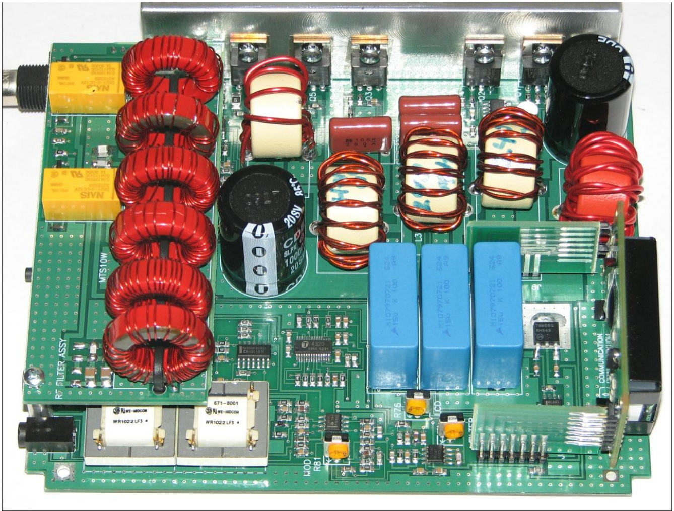
MTS10W Inside View Side
