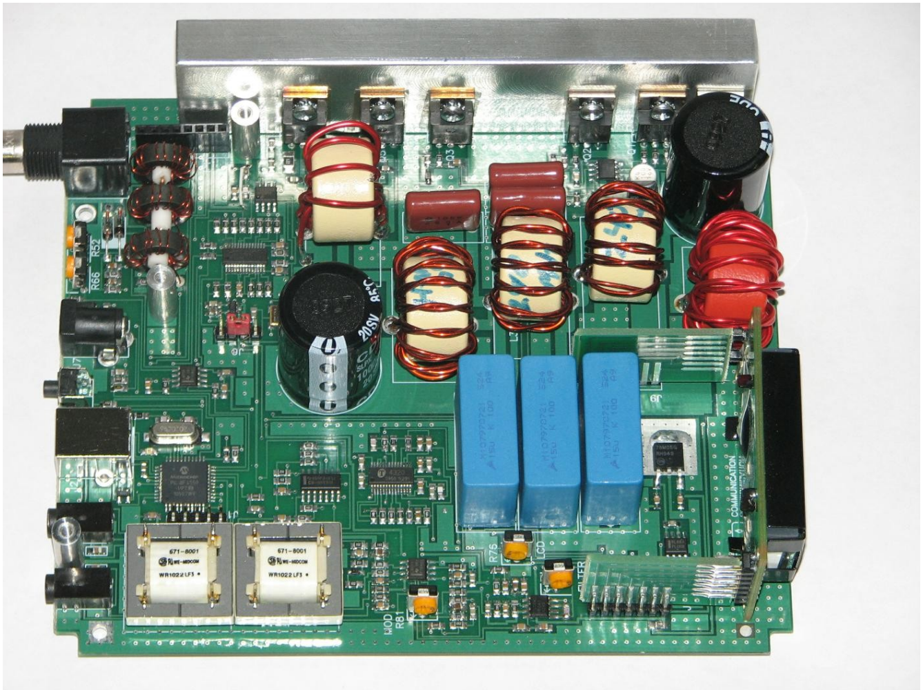
MTS10W Main PCB Assembly, Top View
