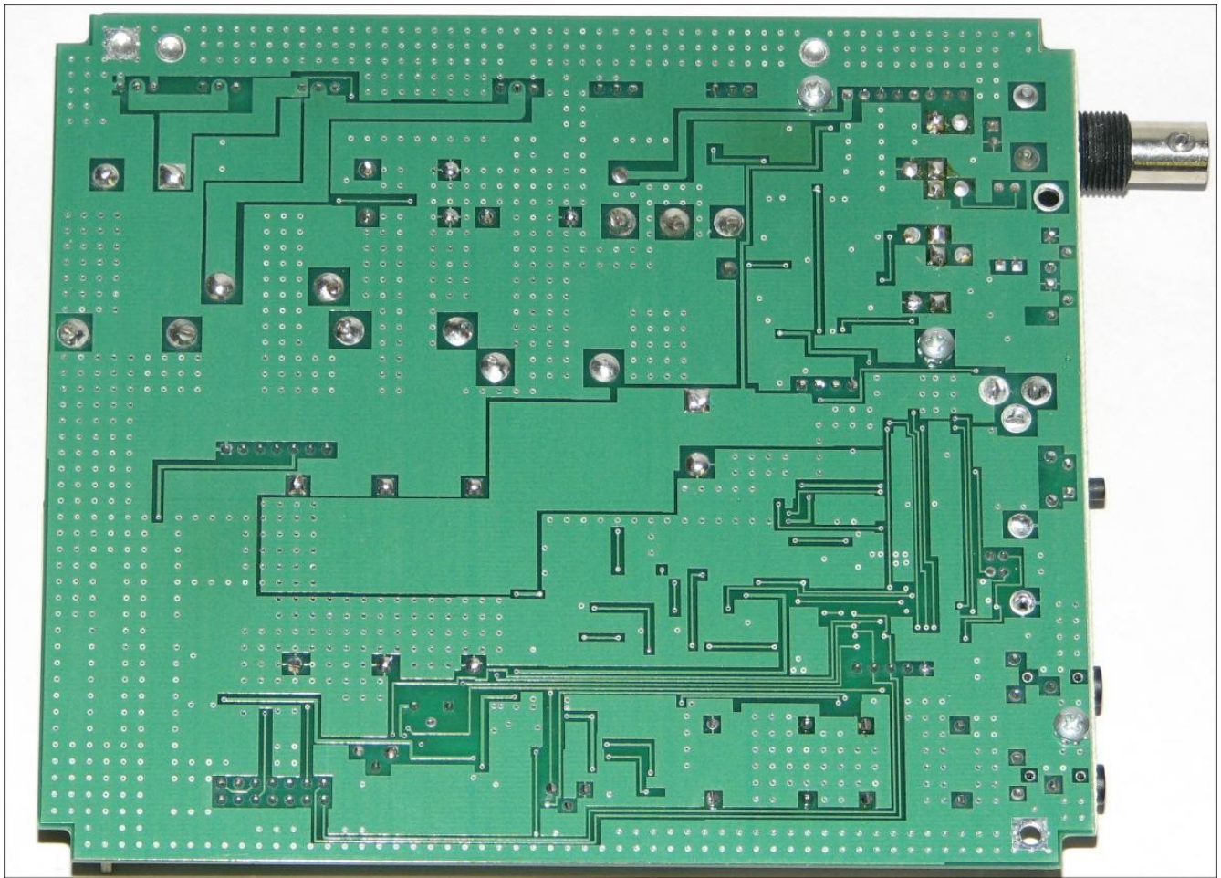
MTS10W Main PCB Assembly Bottom View
