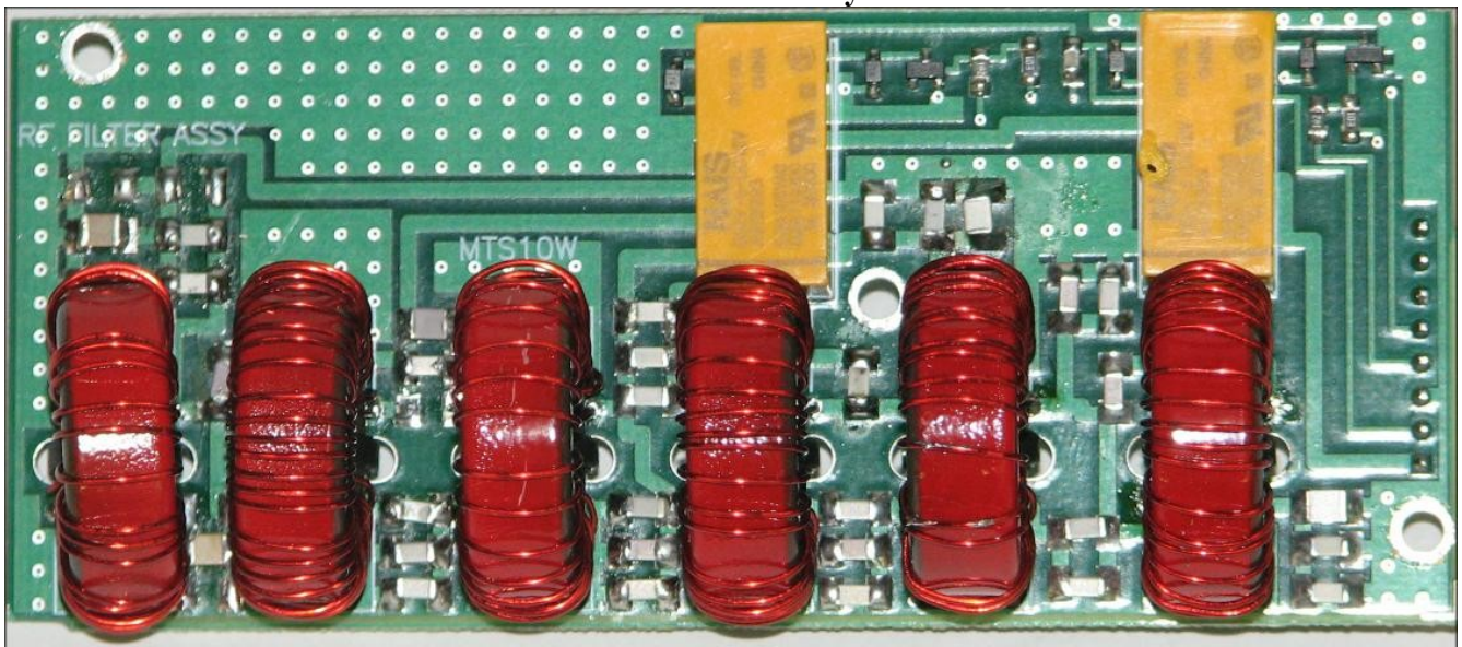
MTS10W Filter Assembly Top View
