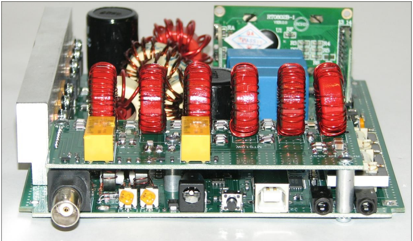
MTS10W Inside View Rear
