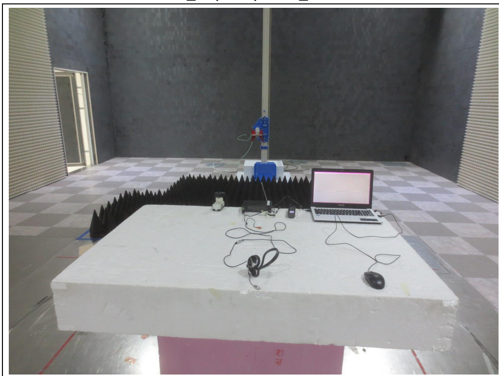
WS1095 _ < (1 ~ 6) GHz _ MODE 2 >
