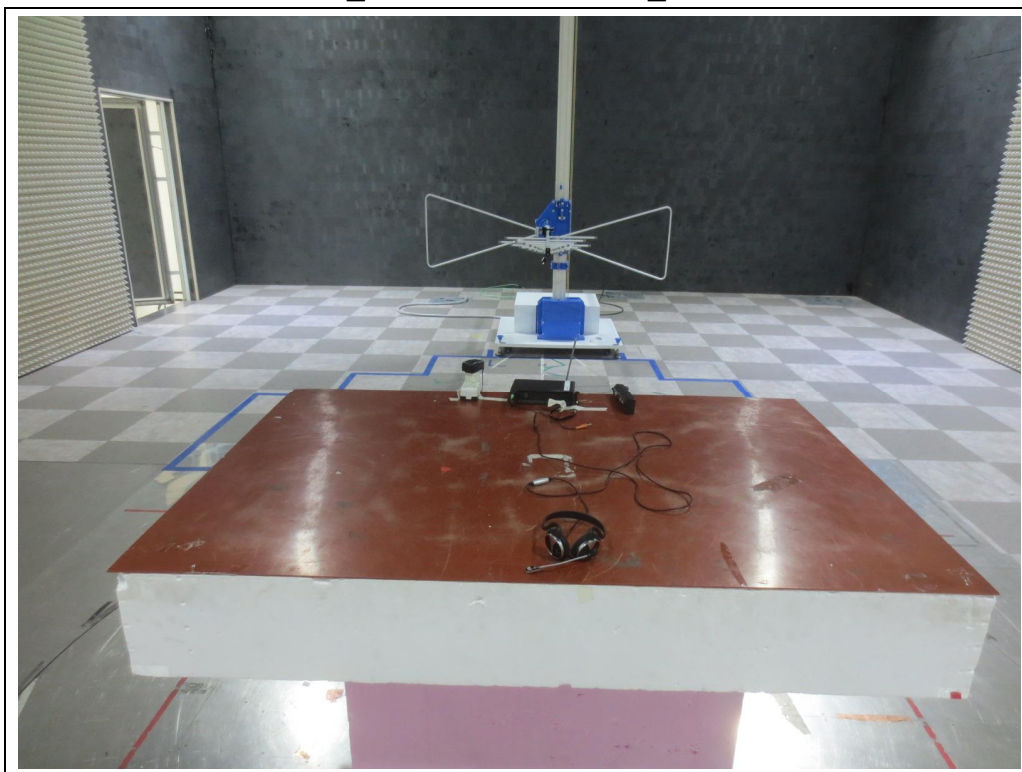
WS1095 _ < 30 MHz ~ 1 GHz _ MODE 1 >
