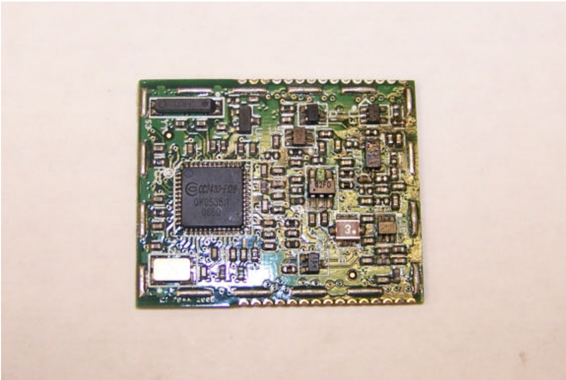
Photo 2. Top of EUT, shield removed
