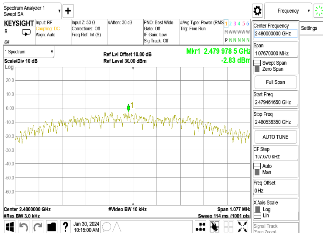
PSD_BLE 1M_HighCH39-2480MHz
