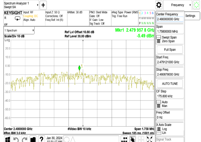
PSD_BLE 2M_HighCH39-2480MHz
