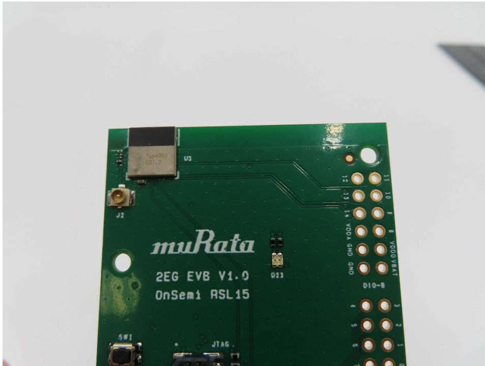
Internal Antenna
