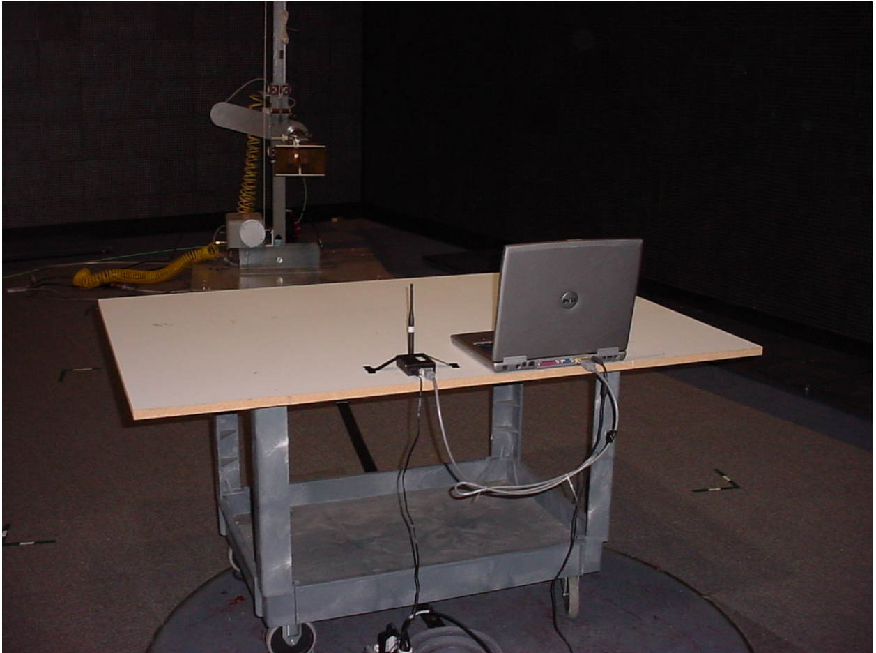
Figure 1: Spurious Emissions Test Setup
