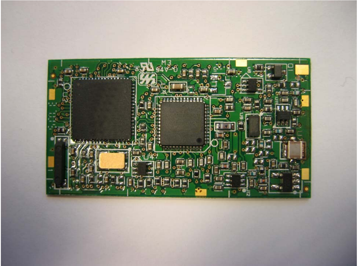
Figure 2: External Photographs – Front View without Shields
