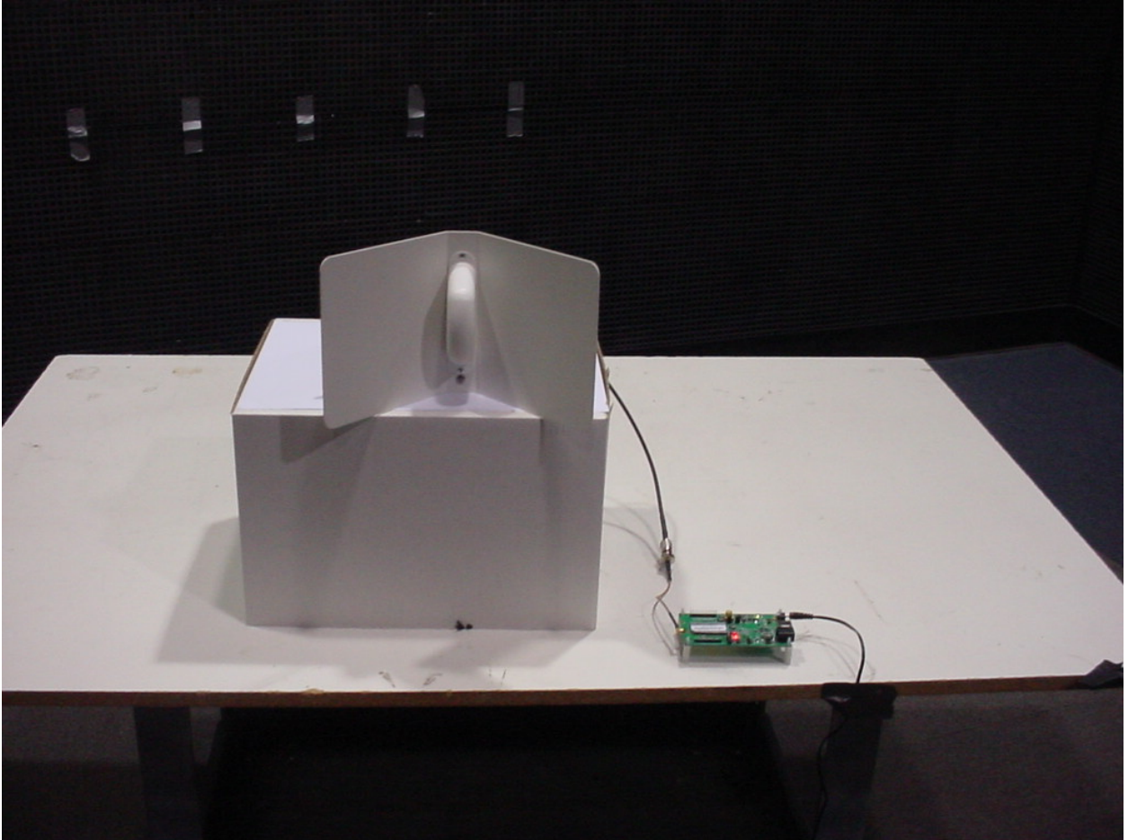
Figure 2: Radiated Emissions – 14dBi Corner Reflector Antenna
