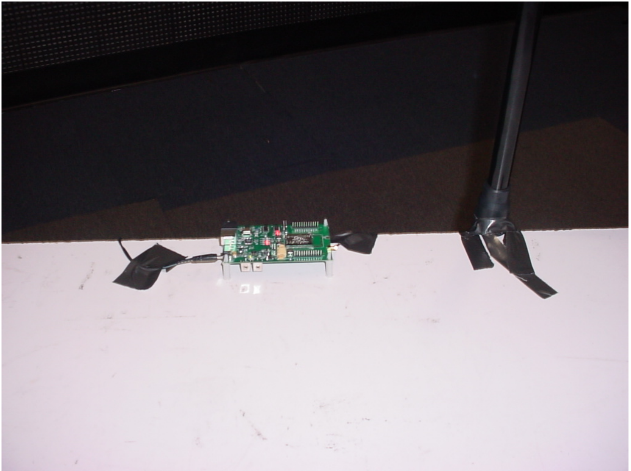
Figure 1: Radiated Emissions – 9dBi Omni-directional Antenna
