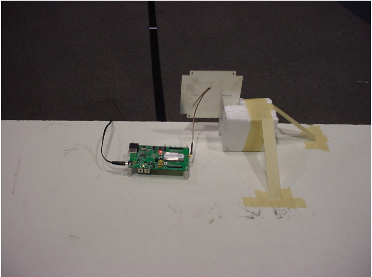
Figure 3: Radiated Emissions – 12dBi Patch Antenna
