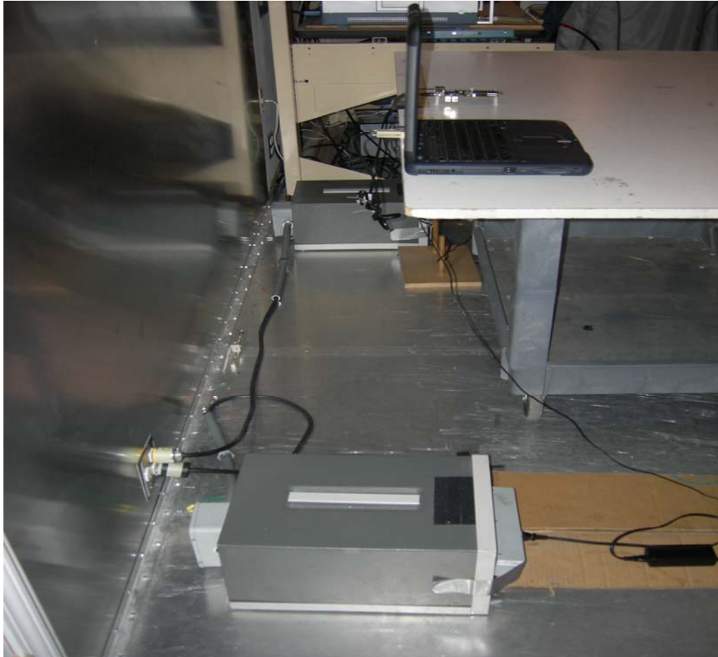
Figure 4: Test Setup Photos – Conducted Emissions
