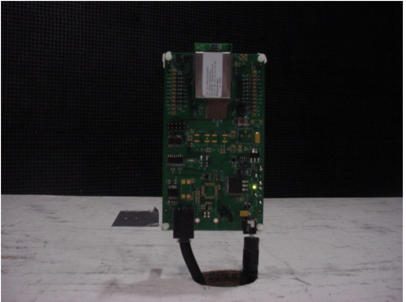
Figure 2: Test Setup Photos – EUT Close Up
