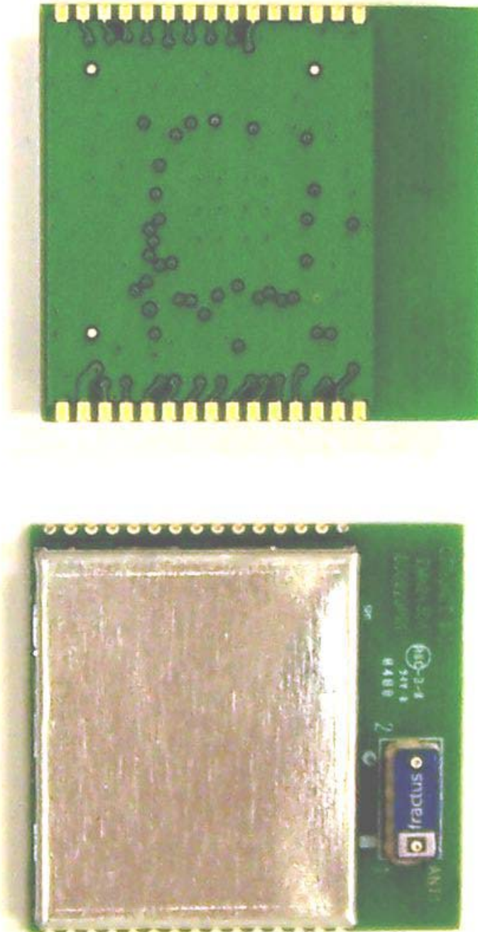
Figure 1: PCB Back and Front with Shields
