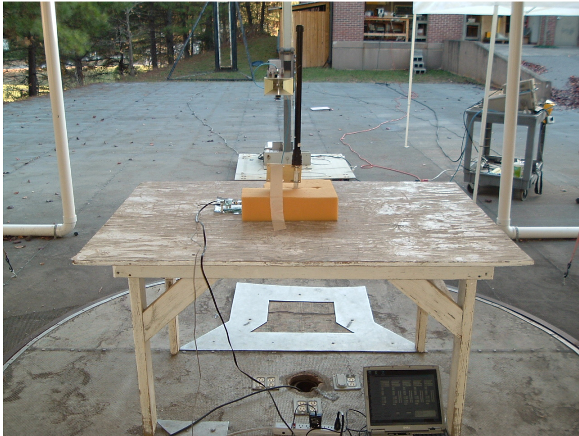
Photograph(s) for Spurious Emissions Omni Antenna Rear
