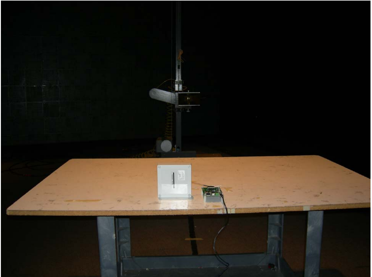
Figure 1: Radiated Emissions – Patch Antenna
