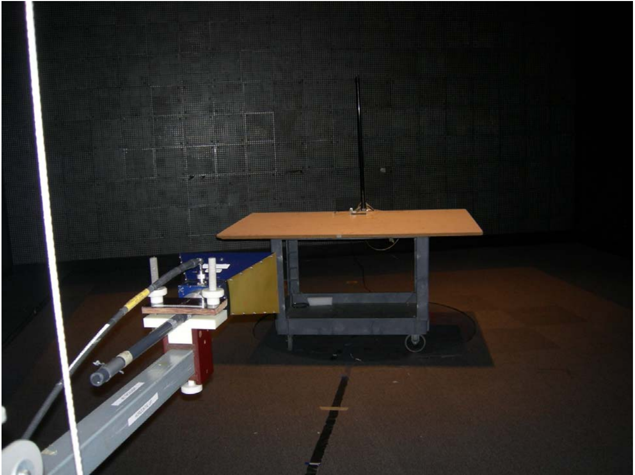
Figure 4: Radiated Emissions – Dipole Antenna
