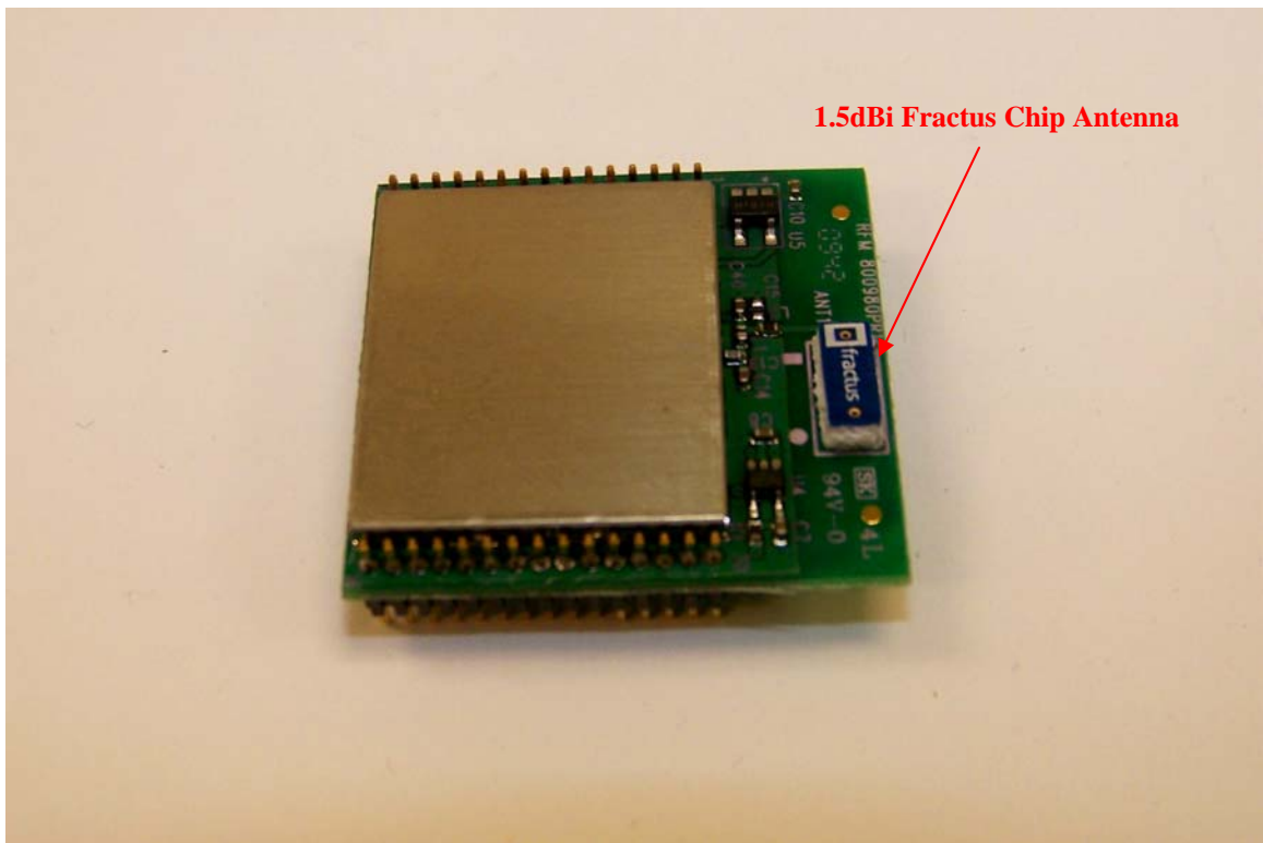
Figure 1: PCB Front (Antenna View)
