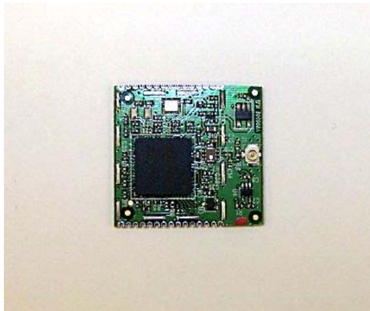
Figure 2: WSN802GC PCB without Shields - Front
