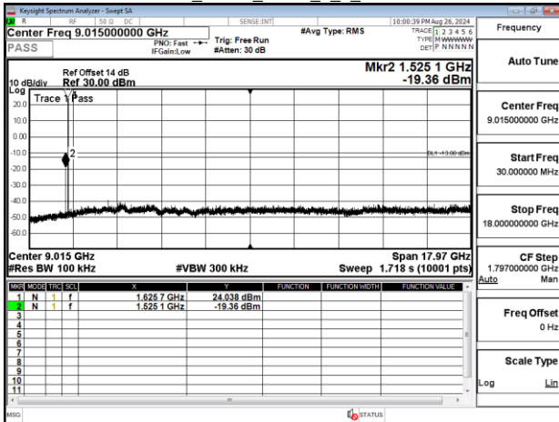
Band255_15kHz_BPSK_1_0_CH261672
