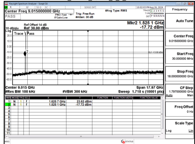
Band255_15kHz_QPSK_1_0_CH261672
