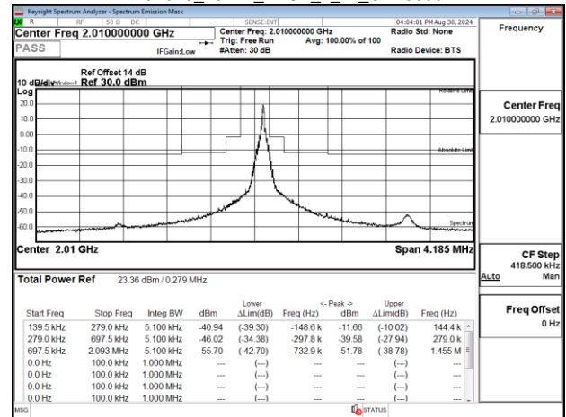
Band23_15kHz_BPSK_1_11_CH25699
