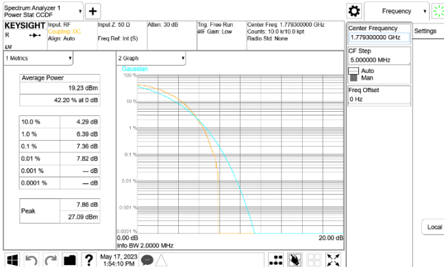
Cat-M1 Band66_1.4MHz_16QAM_RB6_0_CH132665
