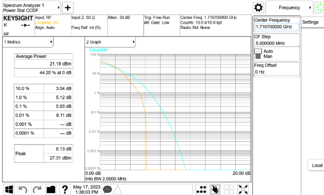
Cat-M1 Band66_1.4MHz_16QAM_RB6_0_CH132322
