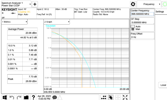
Cat-M1 Band71_5MHz_16QAM_RB6_0_CH133447
