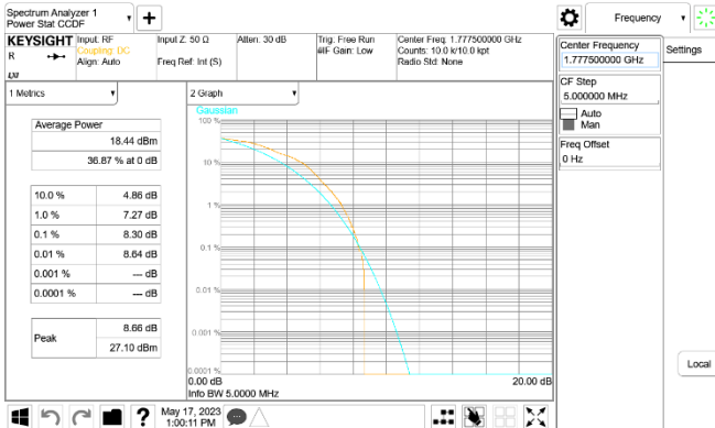
Cat-M1 Band66_5MHz_16QAM_RB6_0_CH132647
