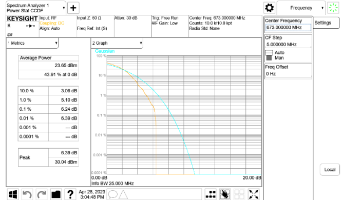
Cat-M1 Band71_20MHz_16QAM_RB6_0_CH133297
