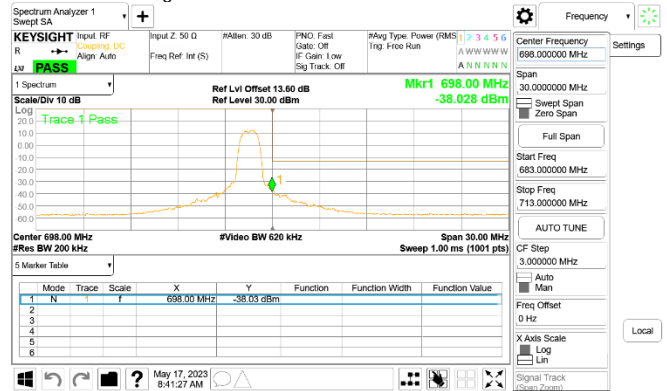
Band Edge_Band71_15MHz_OPSK_RB6_0_CH133397
