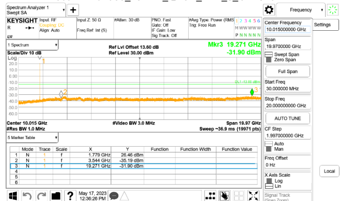
Cat-M1 Band66_10MHz_QPSK_RB1_0_CH132622
