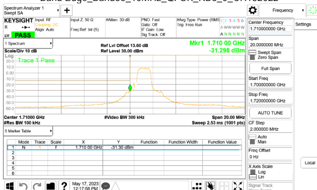
Band Edge_Band66_10MHz_QPSK_RB6_0_CH132022
