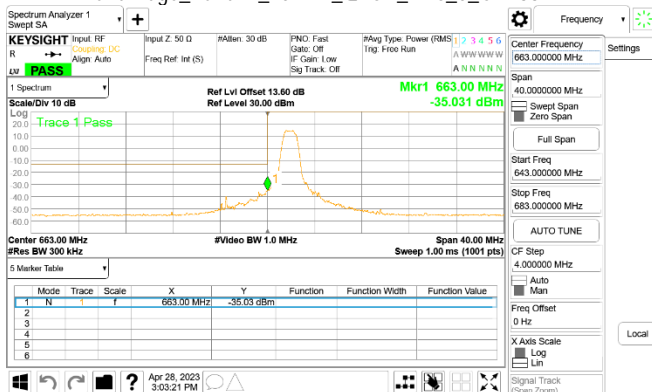
Band Edge_Band71_20MHz_OPSK_RB6_0_CH133222
