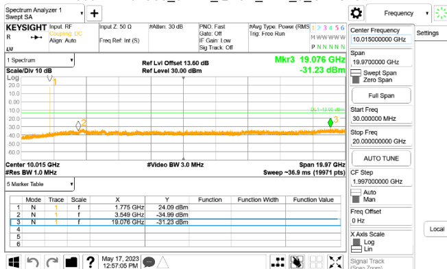
Cat-M1 Band66_5MHz_QPSK_RB1_0_CH132647
