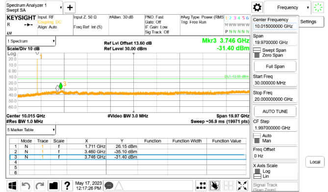
Cat-M1 Band66_10MHz_QPSK_RB1_0_CH132322
