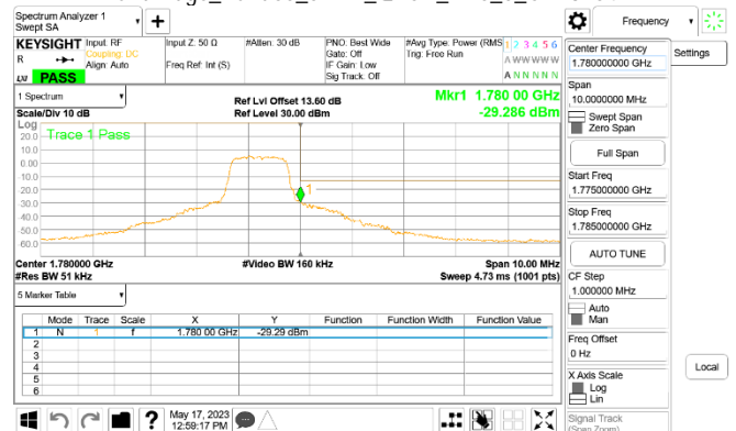
Band Edge_Band66_5MHz_QPSK_RB6_0_CH132647
