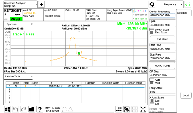
Band Edge_Band71_20MHz_OPSK_RB6_0_CH133372
