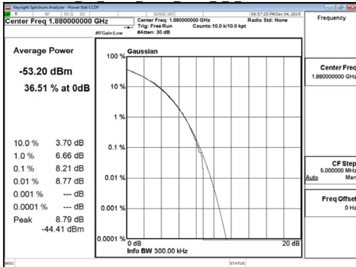
NB IoT Band2 15kHz BPSK 1 0 CH19198
