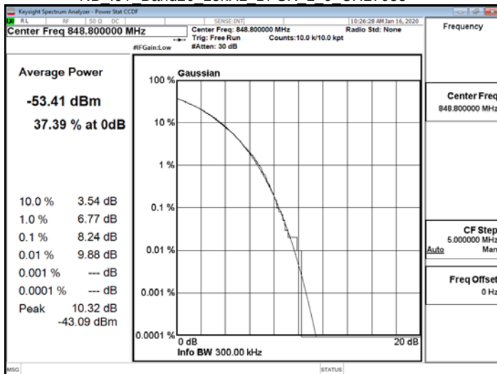
NB IoT Band26 15kHz BPSK 1 0 CH27038
