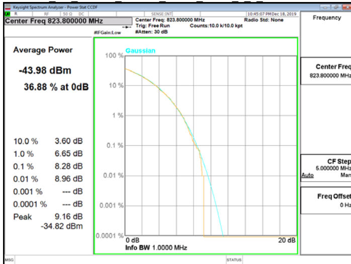
NB IoT Band26 Part90s 15kHz BPSK 1 0 CH26788
