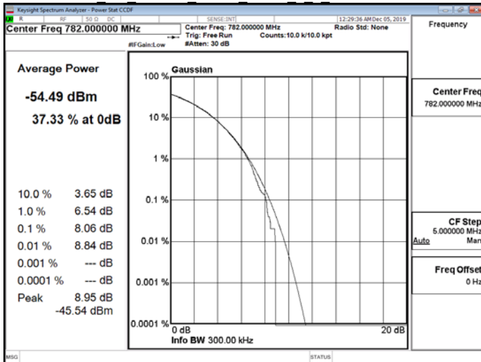
NB IoT Band13 15kHz BPSK 1 0 CH23278
