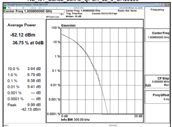
NB IoT Band2 15kHz QPSK 12 0 CH19198
