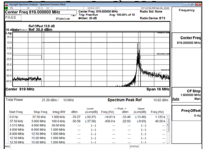
NB IoT Band26 Part90s 15kHz QPSK 12 0 CH26692
