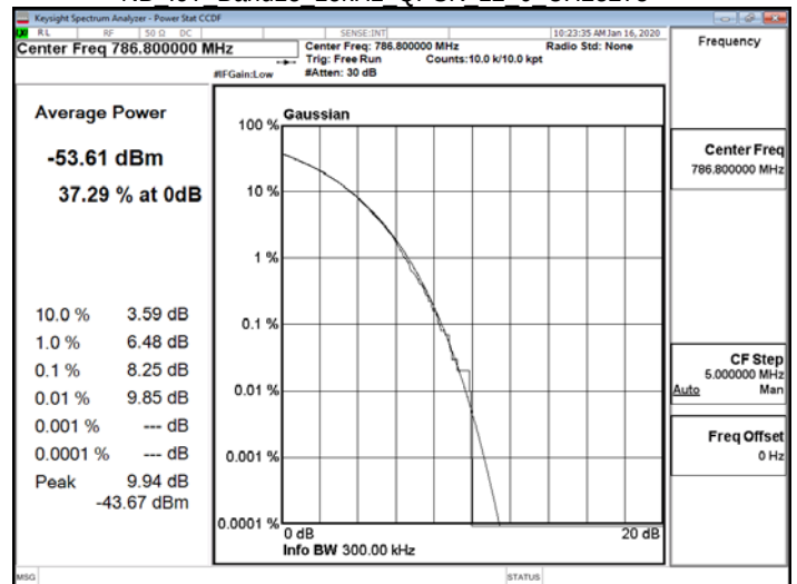
NB IoT Band13 15kHz QPSK 12 0 CH23278
