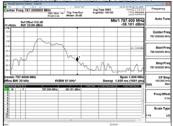
NB IoT Band Edge/NB IoT Band13 15kHz QPSK 12 0 CH23278
