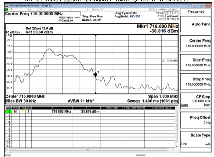
NB IoT_Band Edge\NB IoT\Band17 15kHz QPSK 12 0 CH23848
