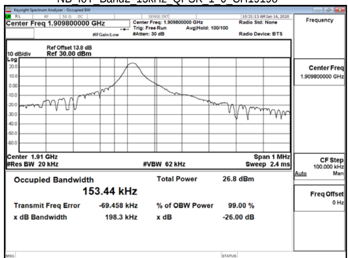
NB IoT Band2 15kHz QPSK 1 0 CH19198
