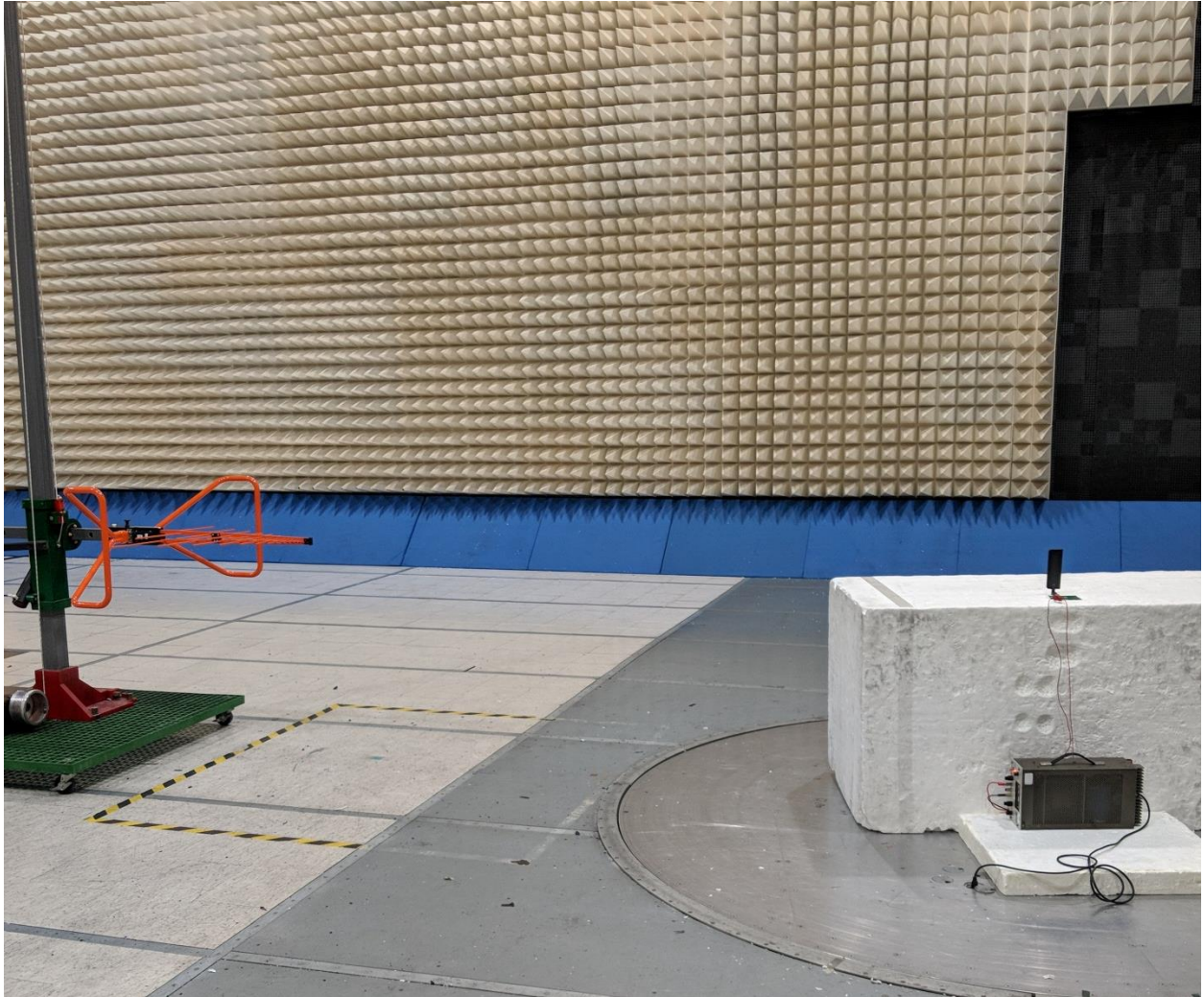
Radiated Spurious Emissions
