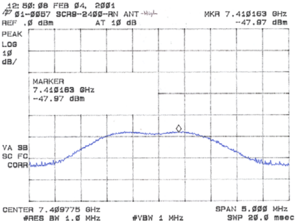
Figure 31 Peak Radiated Spurious Emission 15.247(c) High-Mobility Mark 9 dBi Corner Reflector
