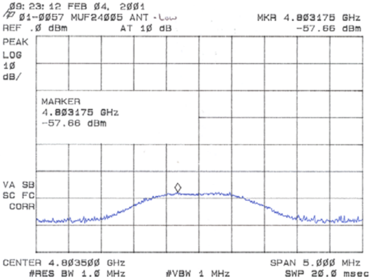
Figure 3m Peak Radiated Spurious Emission 15.247(c) Low – MaxRad 5 dBi Whip
